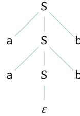
FIGURE 62, FOR QUESTION III.2.21: Parse tree for a^2b^2 .
