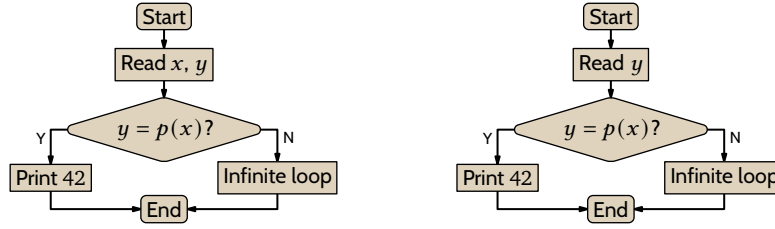
FIGURE 53, FOR QUESTION II.9.11: Flowcharts outlining the machine \mathcal{P}_m that halts only on the m -th prime number.
