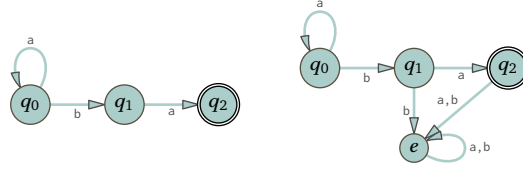
FIGURE 91, FOR QUESTION IV.3.33: Finite State machine for a^*ba .
