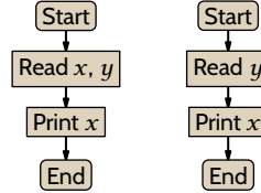
FIGURE 55, FOR QUESTION II.9.15: Flowcharts for \phi_{e_0} and \phi_{s(e_0, x)} , for the machine that outputs its own index.
