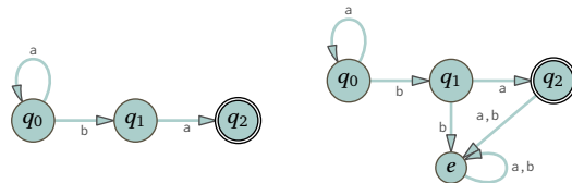
FIGURE 88, FOR QUESTION IV.3.33: Finite State machine for a^*ba .
