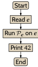
FIGURE 28, FOR QUESTION II.5.31: A single machine whose domain is undecidable.
