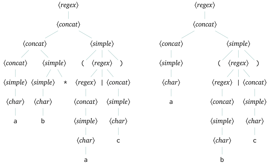
FIGURE 90, FOR QUESTION IV.3.38: Parse trees for a(b|c) and ab^*(a|c) .
