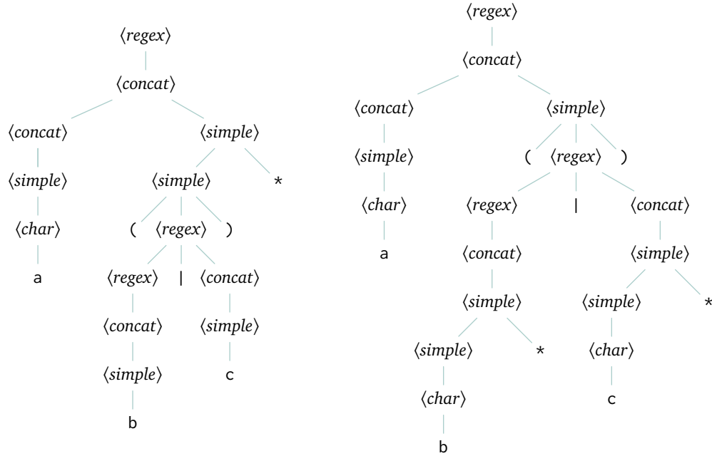
FIGURE 91, FOR QUESTION IV.3.39: Parse trees for a(b|c)^* and a(b^*|c^*) .
