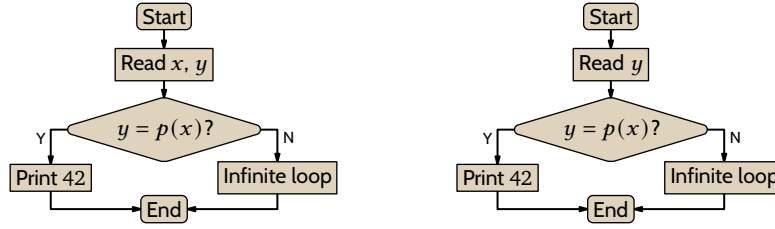
FIGURE 53, FOR QUESTION II.9.11: Flowcharts outlining the machine for \psi = \phi_{e_0} and the machine for \phi_{s(e_0, x)} .
