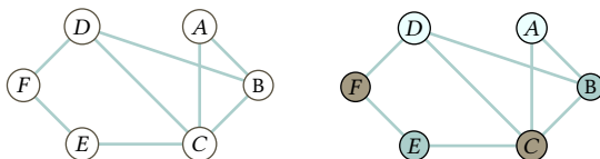
FIGURE 73, FOR QUESTION III.3.24: Relation of incompatibility between fish species.
