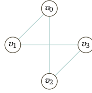
FIGURE 76, FOR QUESTION III.3.30: Graph associated with the given matrix.
