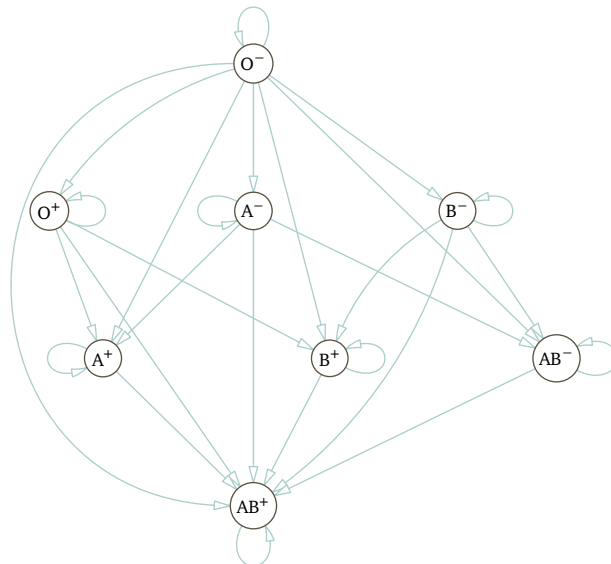
FIGURE 75, FOR QUESTION III.3.27: Compatibility for blood types.
