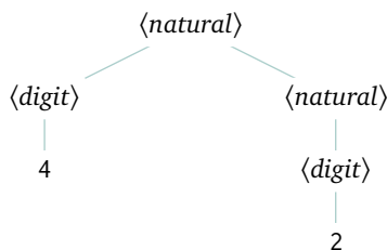
FIGURE 60, FOR QUESTION III.2.14: Parse tree for 42.
