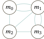
FIGURE 66, FOR QUESTION III.3.16: Bridge connection relation between land masses.
