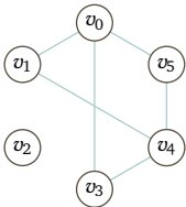
FIGURE 68, FOR QUESTION III.3.18: A graph with some edges.
