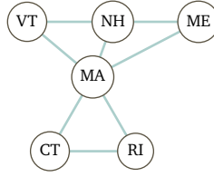
FIGURE 63, FOR QUESTION III.3.16: Adjacency relation among the New England states.
