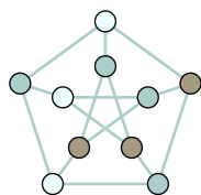
FIGURE 78, FOR QUESTION III.3.35: A 3-coloring of the Petersen graph.
