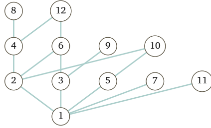
FIGURE 65, FOR QUESTION III.3.16: Divisibility relation among small numbers.
