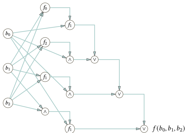
FIGURE 97, FOR QUESTION V.4.33: Directed acyclic graph for the Circuit Evaluation problem.
