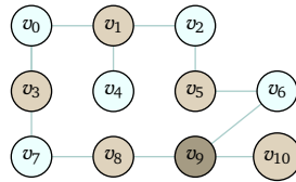
FIGURE 74, FOR QUESTION III.3.25: Cell tower three-coloring.
