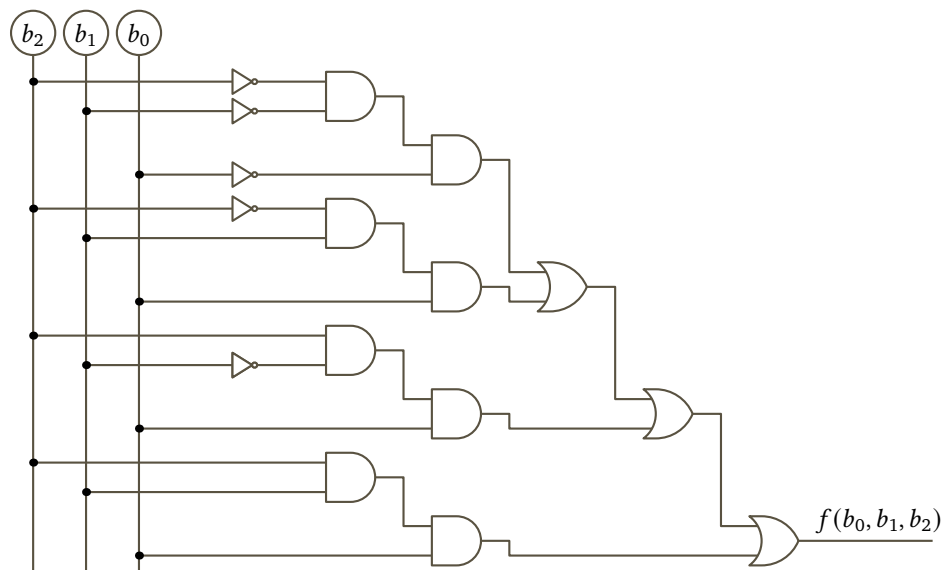
FIGURE 96, FOR QUESTION V.4.33: Initial circuit for the Circuit Evaluation problem.
