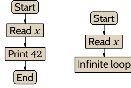
FIGURE 29, FOR QUESTION II.6.24: The machines used to argue that \mathcal{I} is not trivial.
