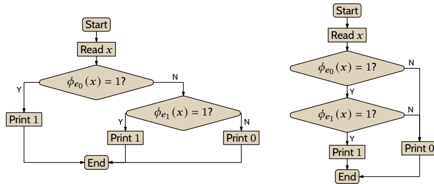
FIGURE 21, FOR QUESTION II.5.39: Sketches of machines to decide union and intersection of decidable languages.
