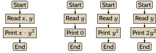
FIGURE 11, FOR QUESTION II.5.16: The machine associated with the function f = \phi_e and machines associated with \phi_{s(e,x)} for x = 0 , x = 1 , and x = 2 .
