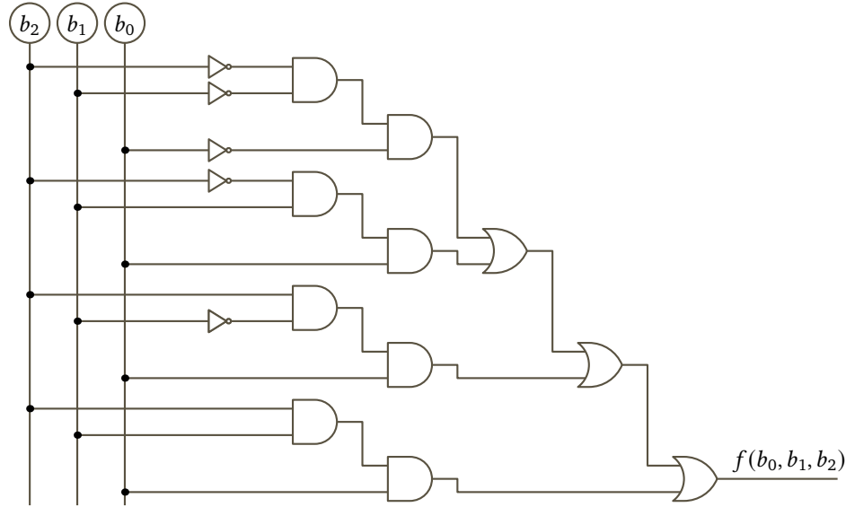
FIGURE 85, FOR QUESTION V.4.33: Initial circuit for the Circuit Evaluation problem.
