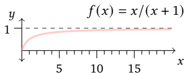
FIGURE 4, FOR QUESTION II.I.39: A correspondence between (0.. \infty) and (0.. 1) .
