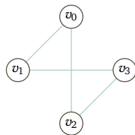
FIGURE 65, FOR QUESTION III.3.30: Graph associated with the given matrix.
