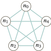
FIGURE 59, FOR QUESTION III.3.19: Complete graph K_5 .
