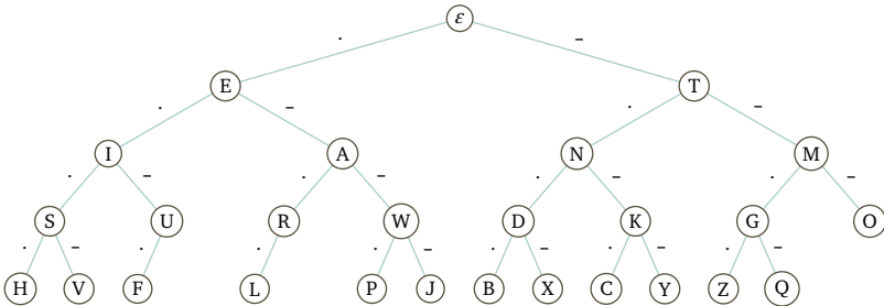
FIGURE 60, FOR QUESTION III.3.20: Prefix relation for Morse code representations of ASCII letters.
