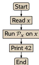
FIGURE 19, FOR QUESTION II.5.29: A single machine that reflects the Halting problem.
