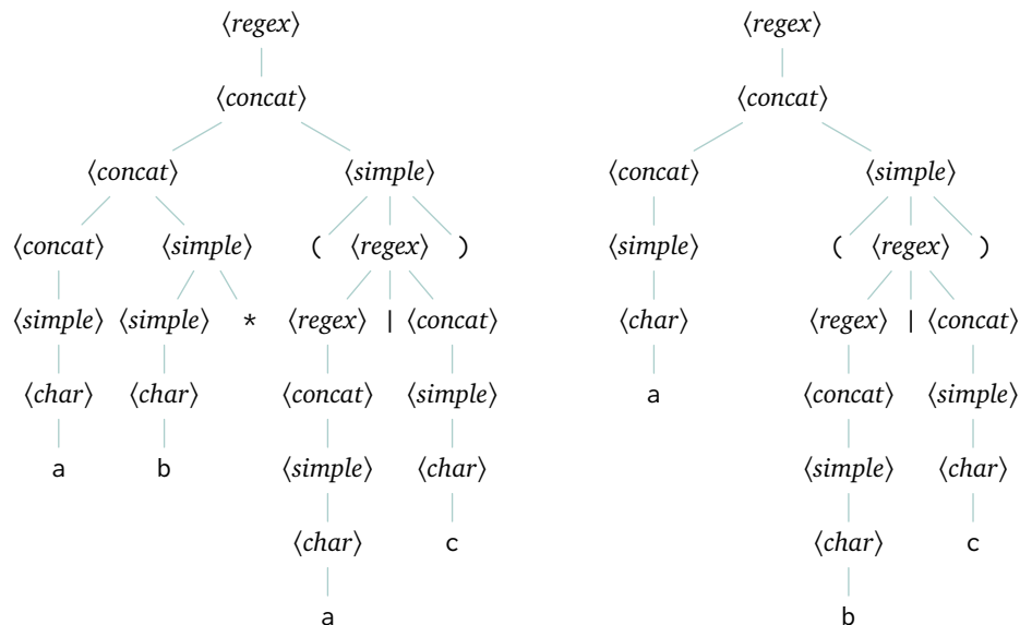
FIGURE 79, FOR QUESTION IV.3.37: Parse trees for a(b|c) and ab^*(a|c) .
