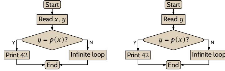
FIGURE 45, FOR QUESTION II.9.10: Flowcharts outlining the machine for \psi = \phi_{e_0} and the machine for \phi_{s(e_0, x)} .
