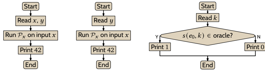
FIGURE 40, FOR QUESTION II.8.26: Computing K with a Tot oracle.
