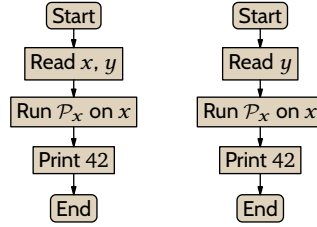
FIGURE 18, FOR QUESTION II.5.24: Outline of the machine for \psi = \phi_{e_0} and the machine for \phi_{s(e_0, x)} .
