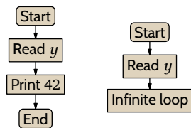
FIGURE 22, FOR QUESTION II.6.16: The machines used to show that the set \mathcal{I} is not trivial.
