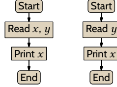
FIGURE 48, FOR QUESTION II.9.15: Flowcharts for \psi = \phi_{e_0} and for \phi_{s(e_0, x)} .
