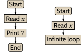
FIGURE 30, FOR QUESTION II.6.24: The machines used to argue that \mathcal{I} is not trivial.
