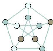
FIGURE 67, FOR QUESTION III.3.35: A 3-coloring of the Petersen graph.
