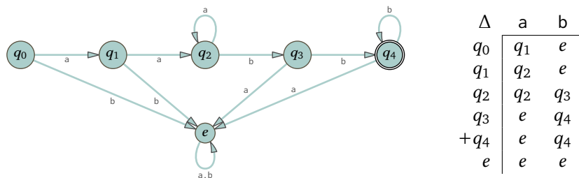
FIGURE 72, FOR QUESTION IV.1.29: Finite State machine for strings of at least two a's and then at least two b's.
