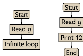
FIGURE 26, FOR QUESTION II.6.20: The machines used to show that \mathcal{I} is not trivial.
