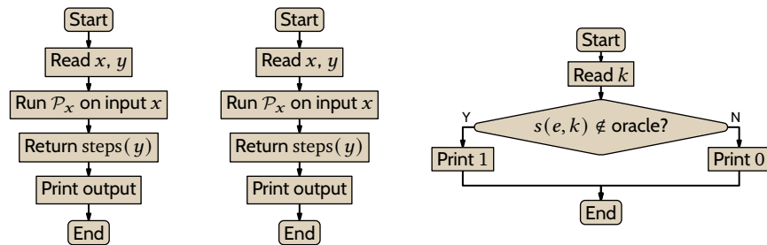
FIGURE 41, FOR QUESTION II.8.27: Computing K with an Ext oracle.
