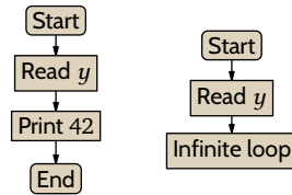
FIGURE 24, FOR QUESTION II.6.18: The machines used to show that the set \mathcal{I} is not trivial.
