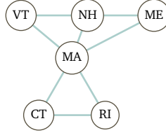
FIGURE 52, FOR QUESTION III.3.16: Adjacency relation among the New England states.
