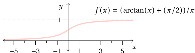
FIGURE 5, FOR QUESTION II.I.42: A correspondence between \mathbb{R} and (0.. 1) .
