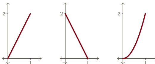
FIGURE 2, FOR QUESTION II.1.32: The correspondences f_0, f_1, f_2: (0..1) \rightarrow (0..2) given by f_0(x) = 2x , f_1(x) = 2-2x , and f_2(x) = 2x^2 .
