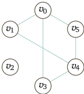
FIGURE 57, FOR QUESTION III.3.18: A graph with some edges.
