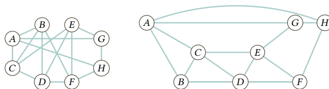
FIGURE 61, FOR QUESTION III.3.22: Drawings of the same graph, with edge crossings and without.
