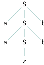
FIGURE 51, FOR QUESTION III.2.22: Parse tree for a^2b^2 .
