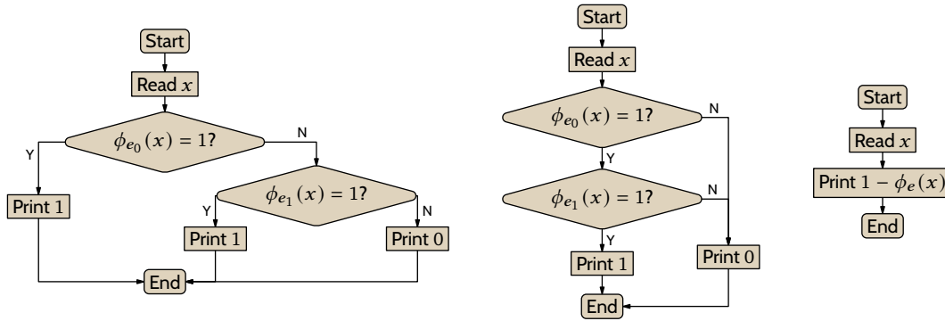
FIGURE 32, FOR QUESTION II.7.32: Machines to decide union, intersection, and complement of computable sets.
