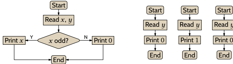
FIGURE 12, FOR QUESTION II.5.16: A sketch of the machine for the function f = \phi_e and of the machines associated with \phi_{s(e,x)} when x = 0 , x = 1 , and x = 2 .
