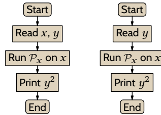
FIGURE 14, FOR QUESTION II.5.19: The machine associated with the function \psi = \phi_{e_0} and the machine associated with \phi_{s(e_0,x)} .
