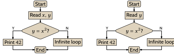
FIGURE 44, FOR QUESTION II.9.9: Flowcharts sketching the machine for \psi = \phi_{e_0} and the machine for \phi_{s(e_0, x)} .
