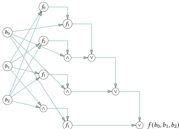
FIGURE 86, FOR QUESTION V.4.33: Directed acyclic graph for the Circuit Evaluation problem.
