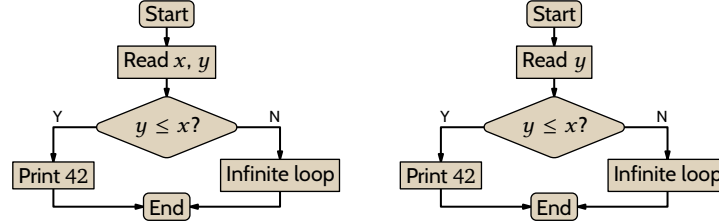
FIGURE 46, FOR QUESTION II.9.12: A sketch of the machine for \psi = \phi_{e_0} , and the machine for \phi_{s(e_0, x)} .
