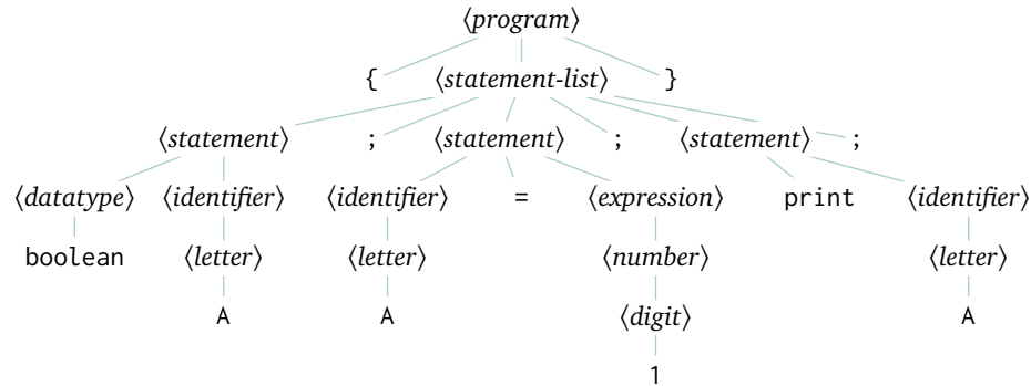
FIGURE 68, FOR QUESTION III.A.9: Parse tree for C-like language.
