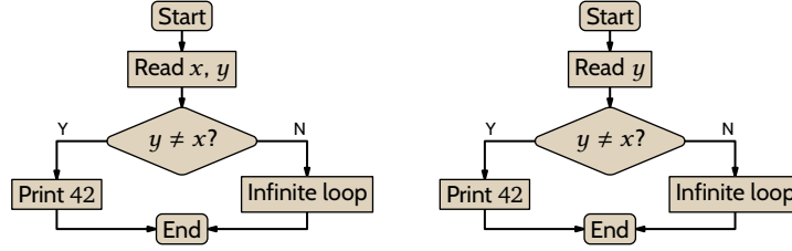
FIGURE 47, FOR QUESTION II.9.14: Sketches for \psi = \phi_{e_0} and for \phi_{s(e_0, x)} .
