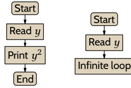
FIGURE 23, FOR QUESTION II.6.17: The machines used to show that the set \mathcal{I} of indices of the squarer function is not trivial.
