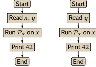
FIGURE 16, FOR QUESTION II.5.21: The machine associated with \psi = \phi_{e_0} and the machine for \phi_{s(e_0, x)} .
