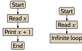
FIGURE 27, FOR QUESTION II.6.21: The machines used to show that \mathcal{I} is not trivial.
