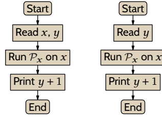
FIGURE 17, FOR QUESTION II.5.23: Sketches of the machine associated with \psi = \phi_{e_0} and the machine associated with \phi_{s(e_0, x)} .
