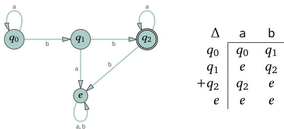
FIGURE 73, FOR QUESTION IV.I.29: Finite State machine for strings with some a's, then two b's, then some a's.
