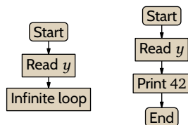
FIGURE 25, FOR QUESTION II.6.19: Outlines of the Turing machines used to show that \mathcal{I} is not trivial.
