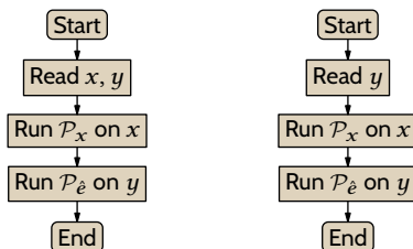
FIGURE 31, FOR QUESTION II.6.33: Sketches of machines for the proof of half of Rice's Theorem.
