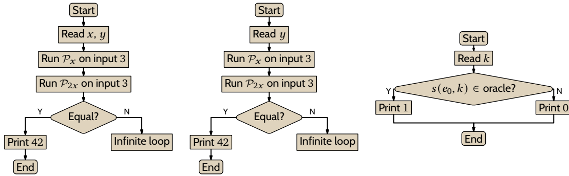
FIGURE 39, FOR QUESTION II.8.25: The set \{x \mid \phi_x(3) \downarrow = \phi_{2x}(3) \downarrow\} is T -equivalent to K .
