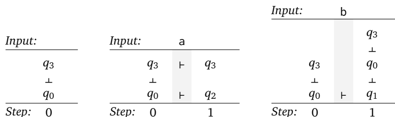
FIGURE 86, FOR QUESTION IV.2.27: Computation trees for the strings \varepsilon , a , and b .
