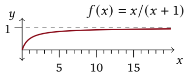
FIGURE 11, FOR QUESTION II.1.39: A correspondence between (0.. \infty) and (0..1) .
