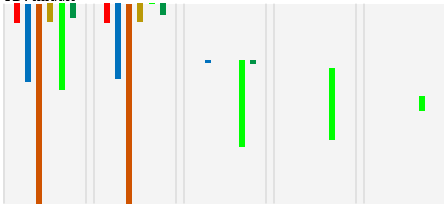
TD: middle
