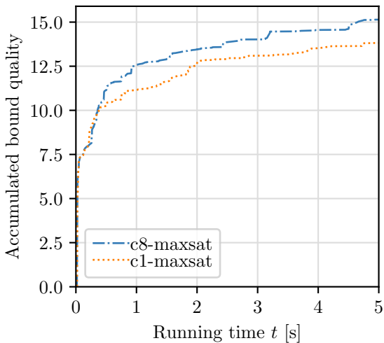
MaxSAT quality progression: ub
