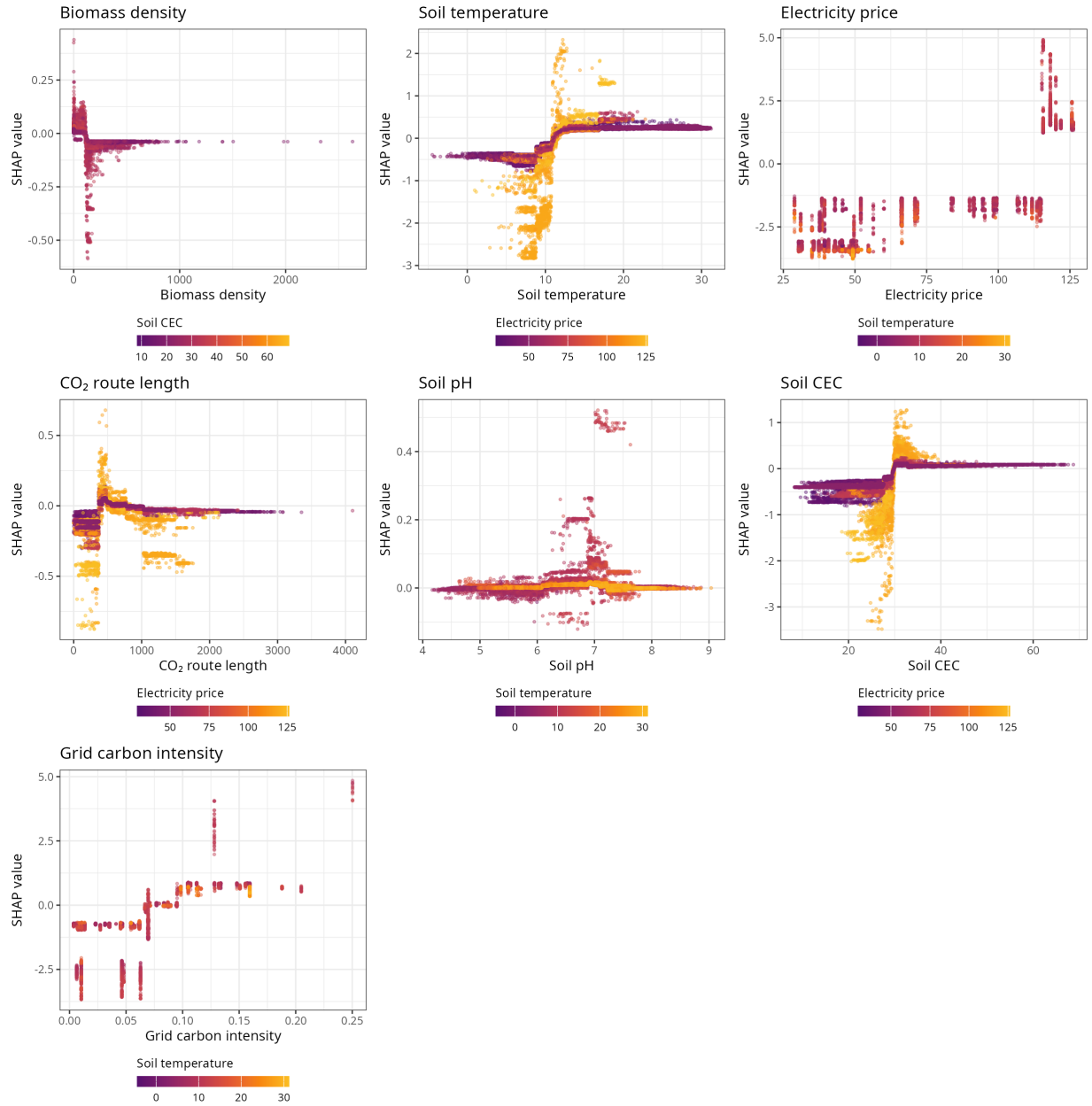
Figure S10: SHAP dependence plots for BES, global model (all regions): SHAP value of each input against its value, coloured by the input with the strongest interaction.
