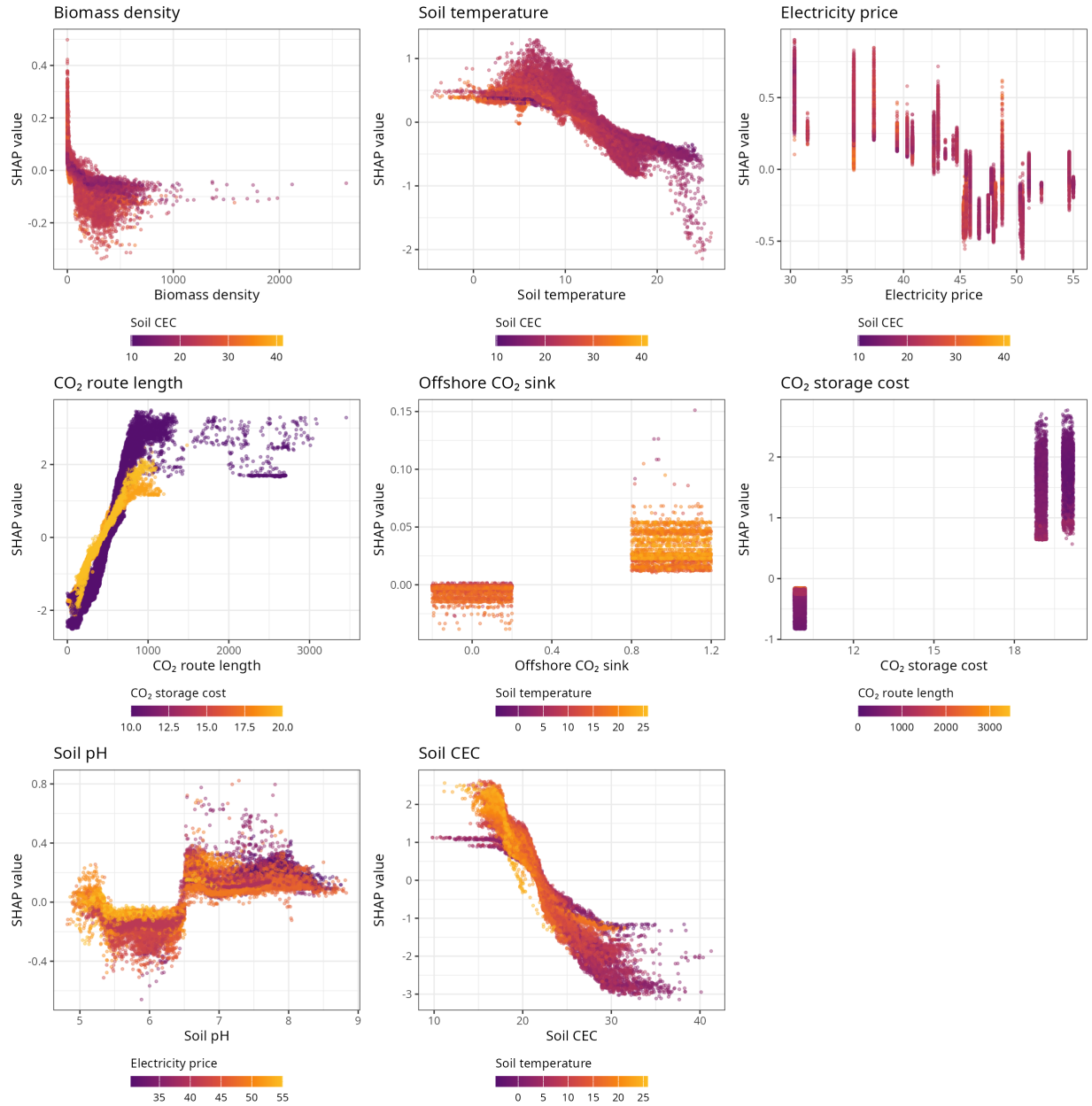
Figure S16: SHAP dependence plots for BEBCS, China model: SHAP value of each input against its value, coloured by the input with the strongest interaction.
