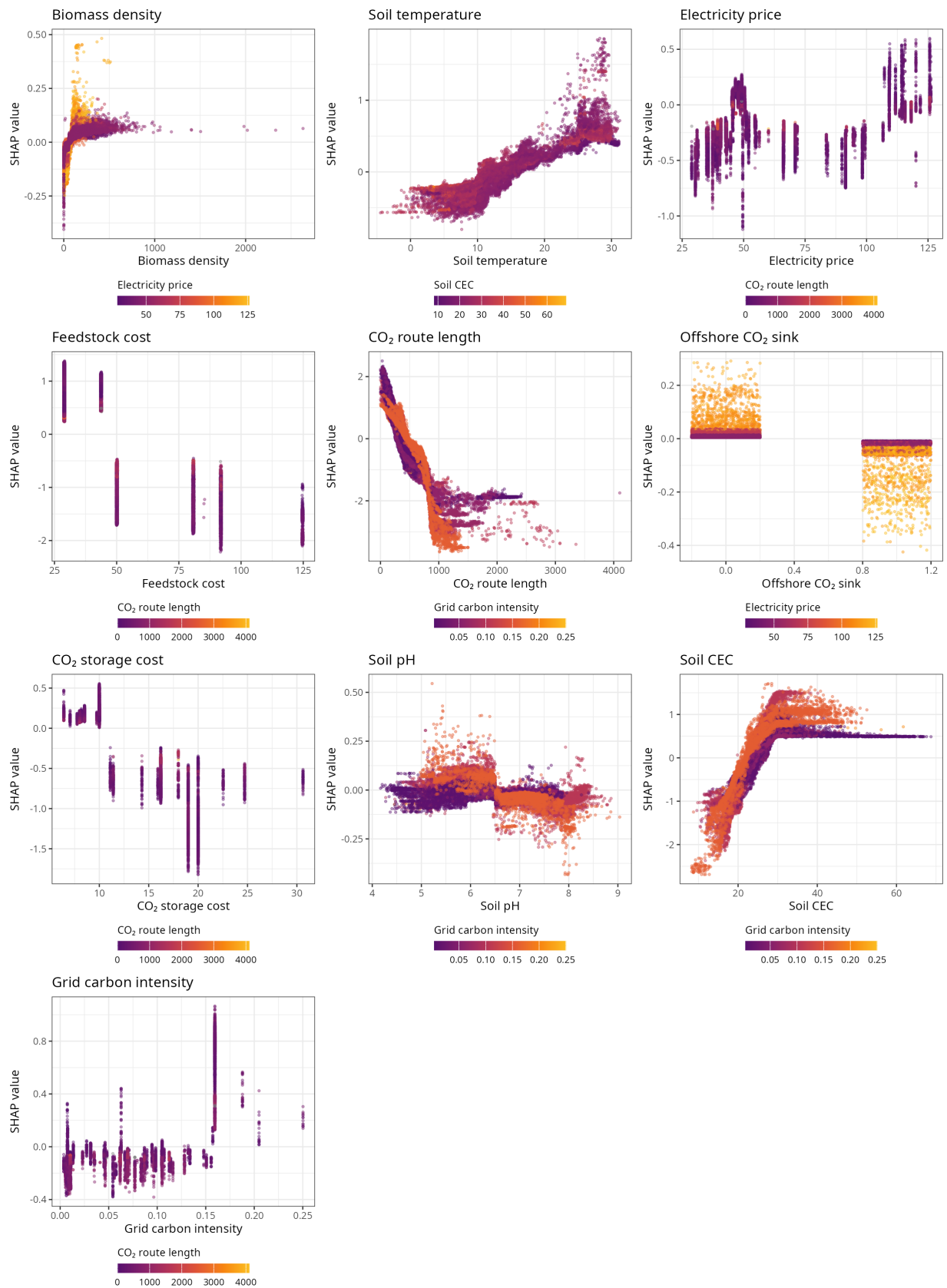
Figure S9: SHAP dependence plots for BECCS, global model (all regions): SHAP value of each input against its value, coloured by the input with the strongest interaction.
