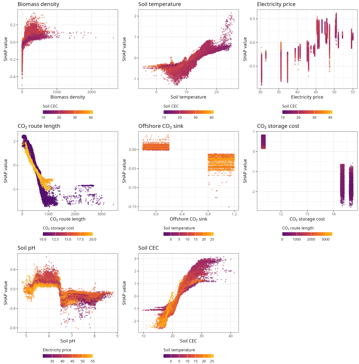
Figure S17: SHAP dependence plots for BECCS, China model: SHAP value of each input against its value, coloured by the input with the strongest interaction.
