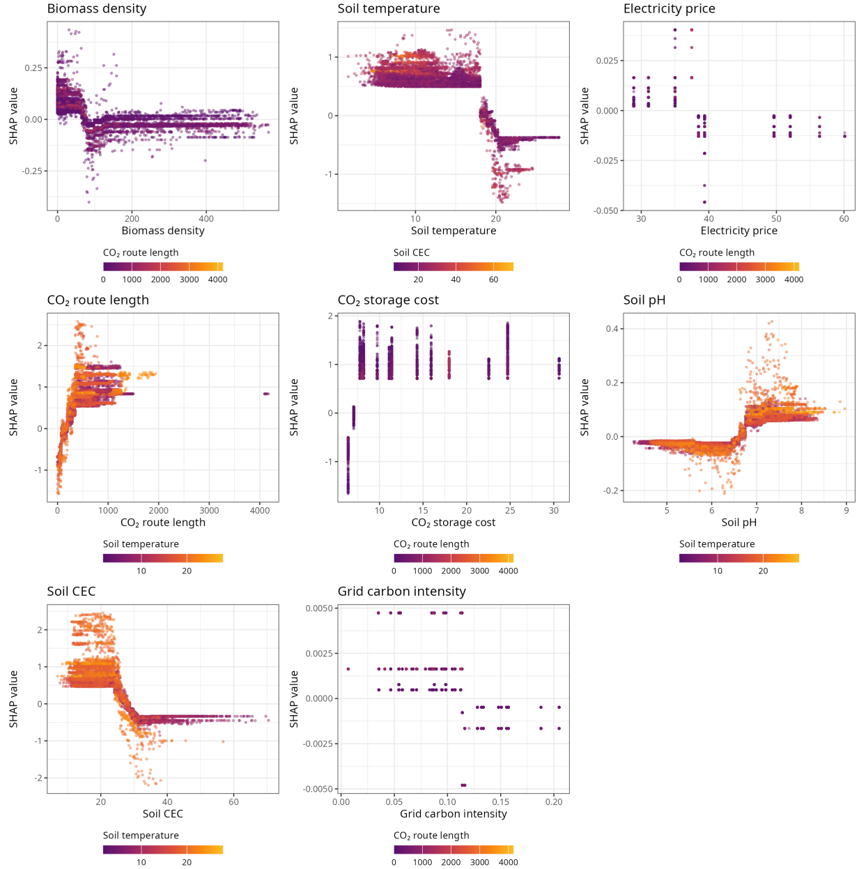
Figure S11: SHAP dependence plots for BEBCS, United States model: SHAP value of each input against its value, coloured by the input with the strongest interaction.
