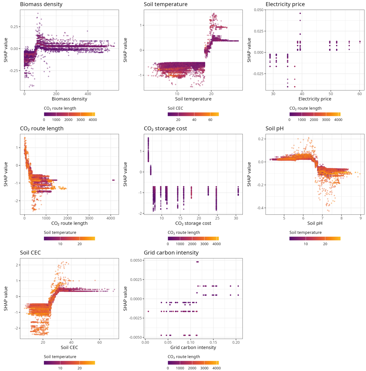
Figure S12: SHAP dependence plots for BECCS, United States model: SHAP value of each input against its value, coloured by the input with the strongest interaction.
