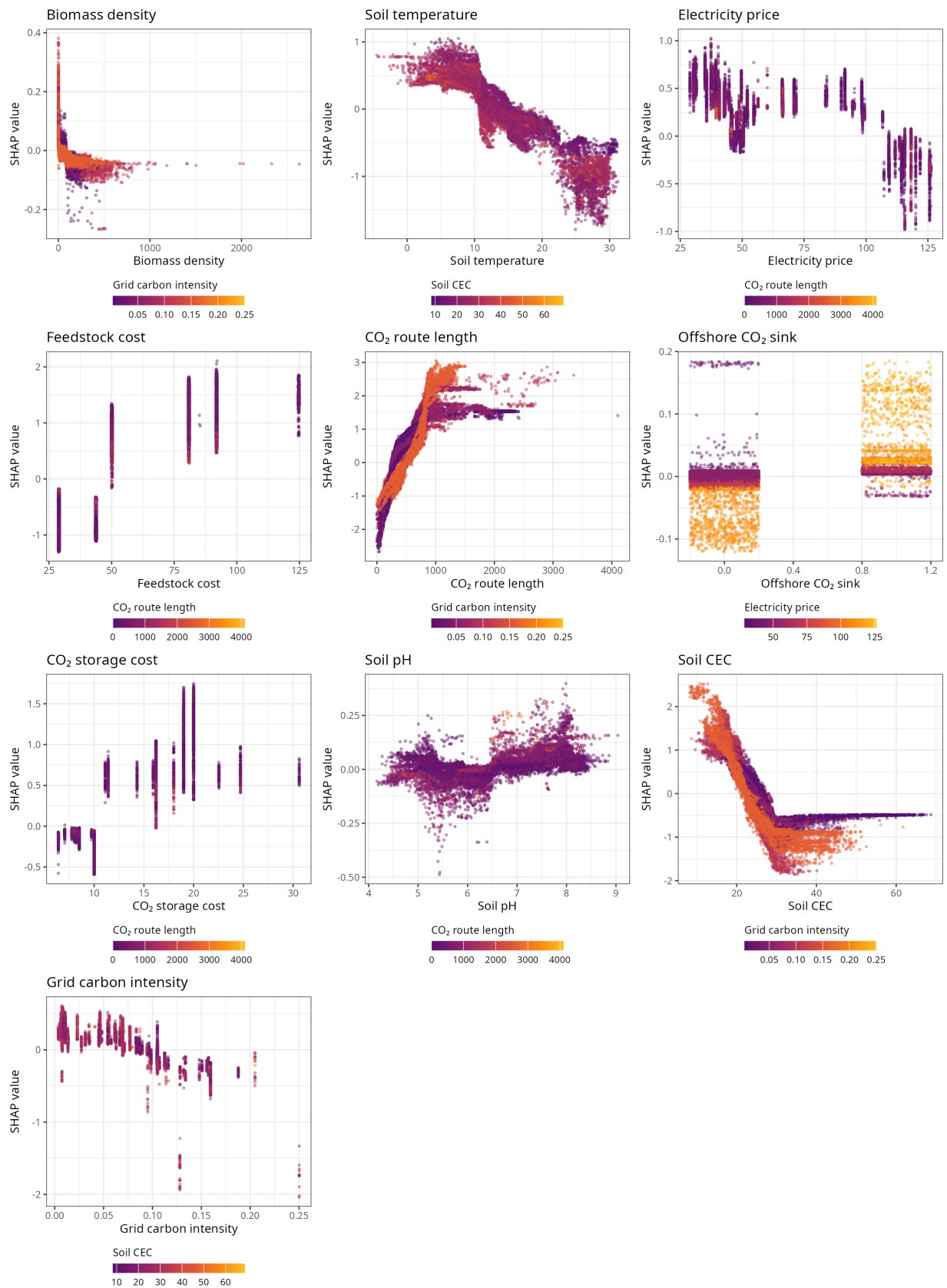
Figure S8: SHAP dependence plots for BEBCS, global model (all regions): SHAP value of each input against its value, coloured by the input with the strongest interaction.
