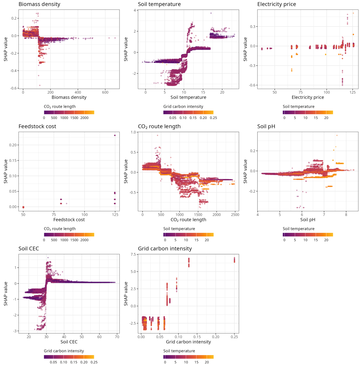
Figure S15: SHAP dependence plots for BES, Europe model: SHAP value of each input against its value, coloured by the input with the strongest interaction.
