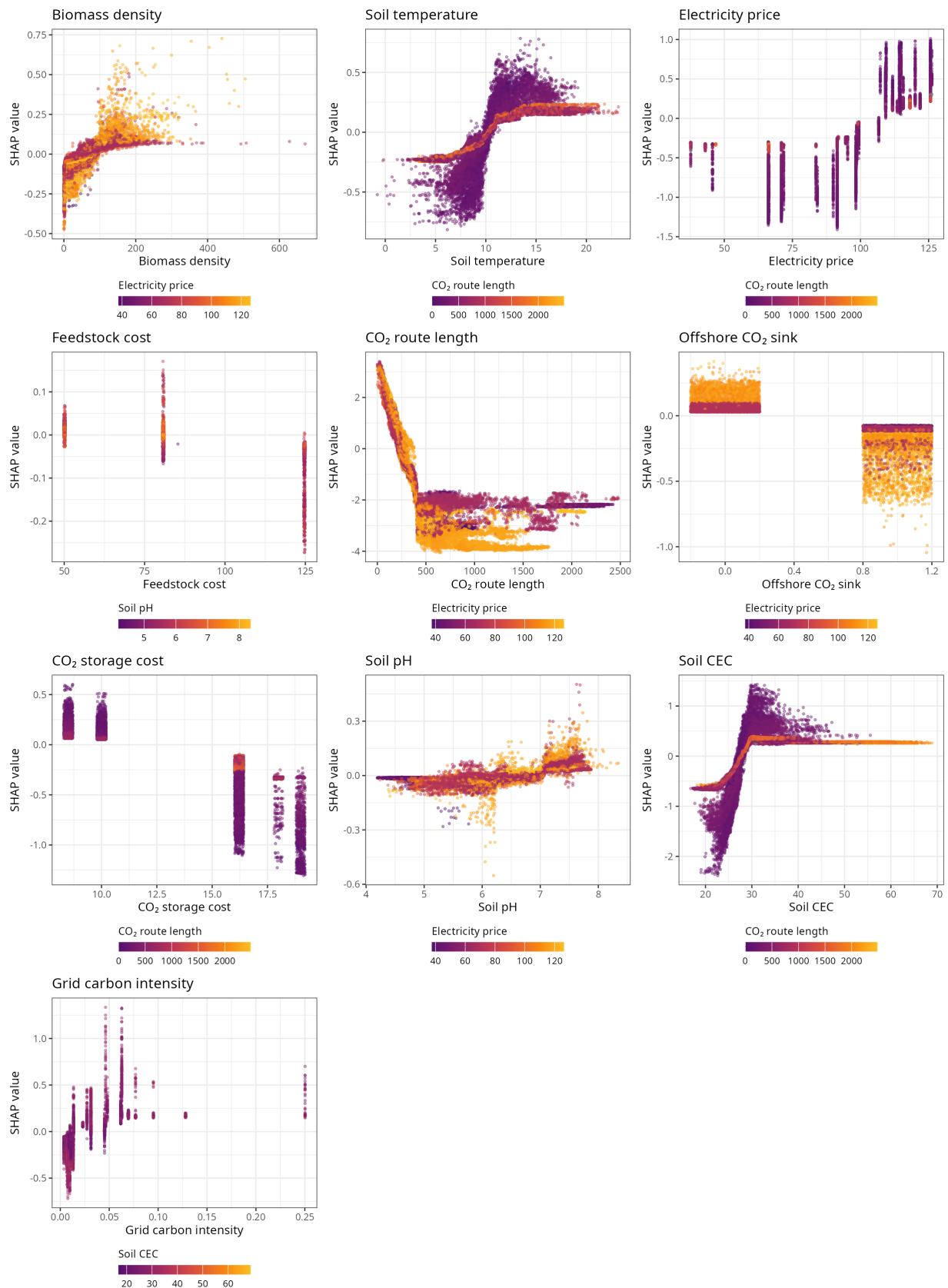
Figure S14: SHAP dependence plots for BECCS, Europe model: SHAP value of each input against its value, coloured by the input with the strongest interaction.
