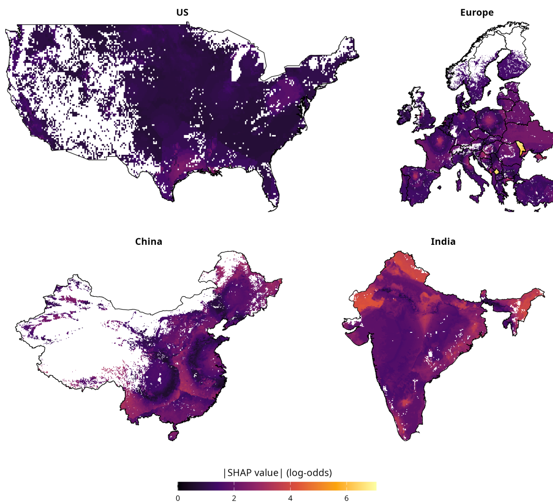
Figure 8: Magnitude (absolute SHAP value, log-odds) of the dominant spatial driver in each grid cell, from the regional surrogate classifiers.
