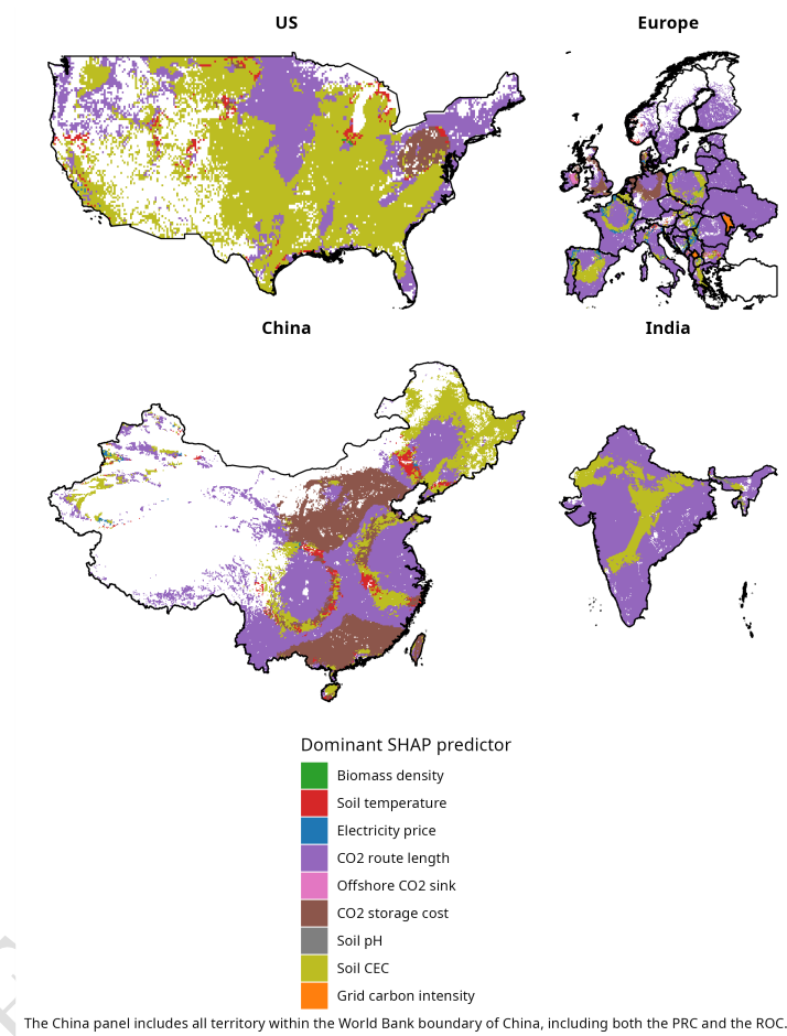
Figure 9: Dominant spatial driver of the optimal technology in each grid cell: the input with the largest absolute SHAP value for the cell's optimal technology, from surrogate classifiers fitted separately for each region (scenario CP100_MW250; see Supplementary Information). The China panel includes all territory within the World Bank boundary of China, including both the PRC and the ROC.
