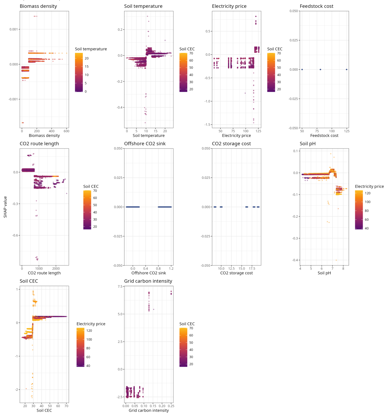
SHAP dependence, Europe model: BES
