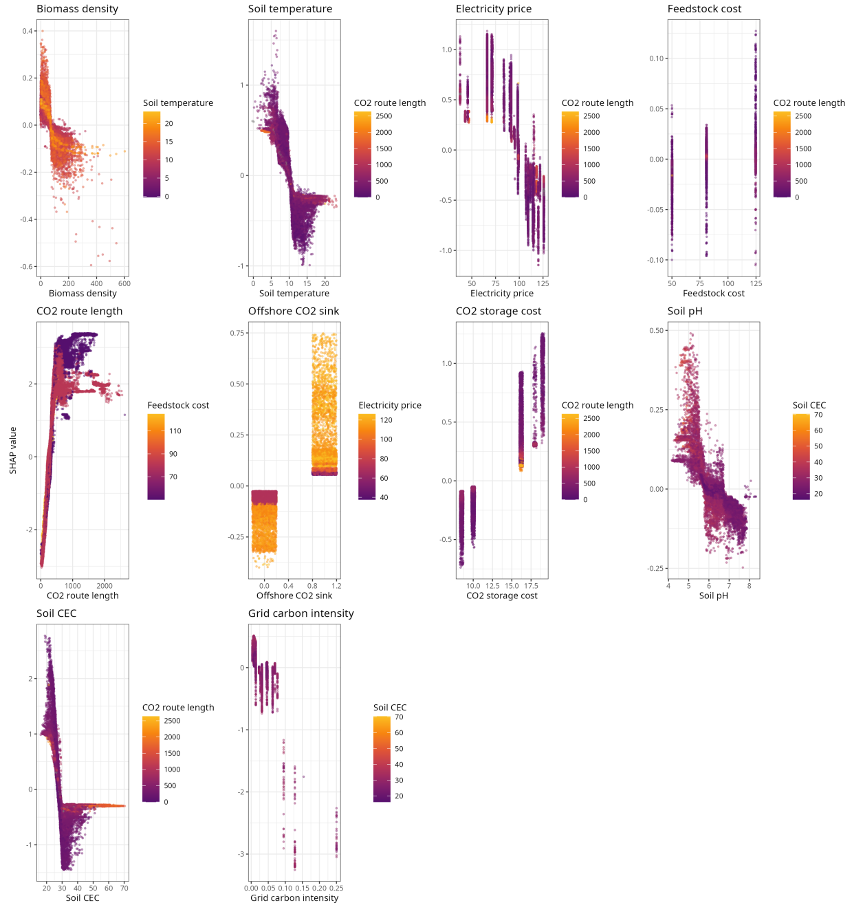
SHAP dependence, Europe model: BEBCS
