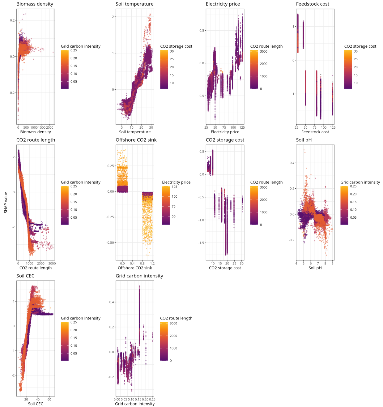
SHAP dependence, Global model: BECCS
