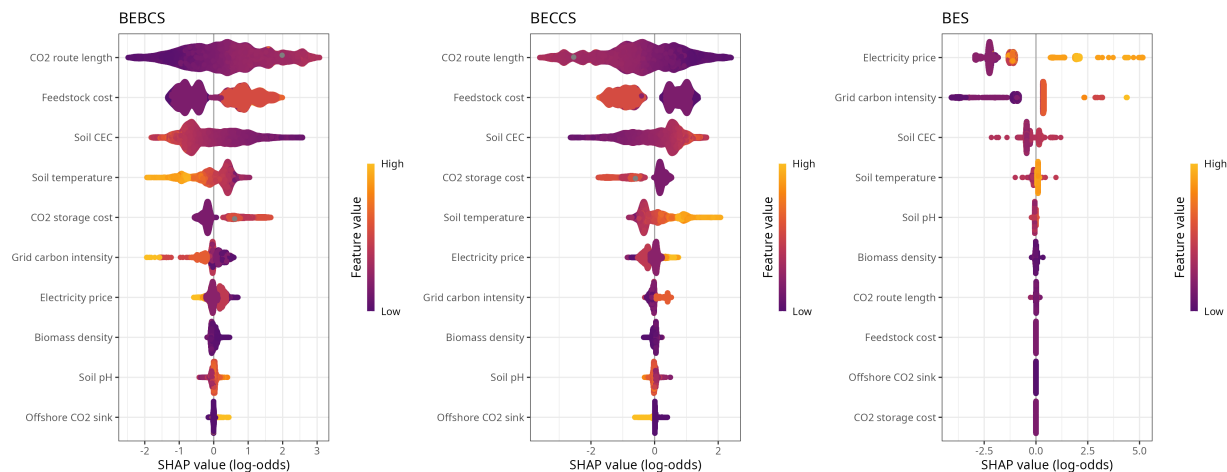
SHAP values for the optimal technology: Global model
