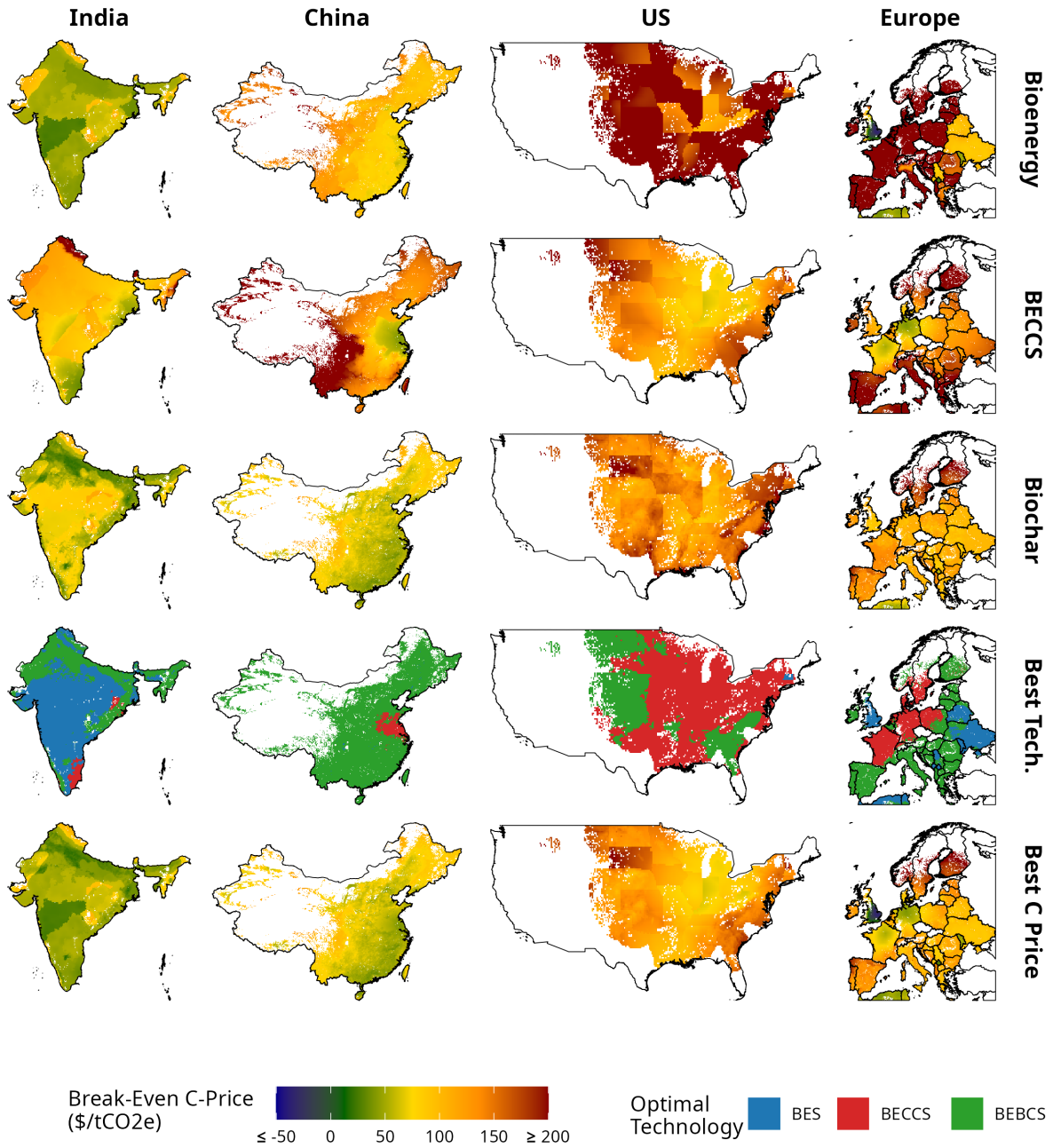
Figure 1: Minimum Break-even carbon price for each technology option. The penultimate row shows the technology with the lowest break-even price, and the final row shows that price. The lowest break-even technology is the first to become profitable as the carbon price rises; it is not necessarily the technology with the highest NPV at a given carbon price (see Figure 2 to Figure 5).
