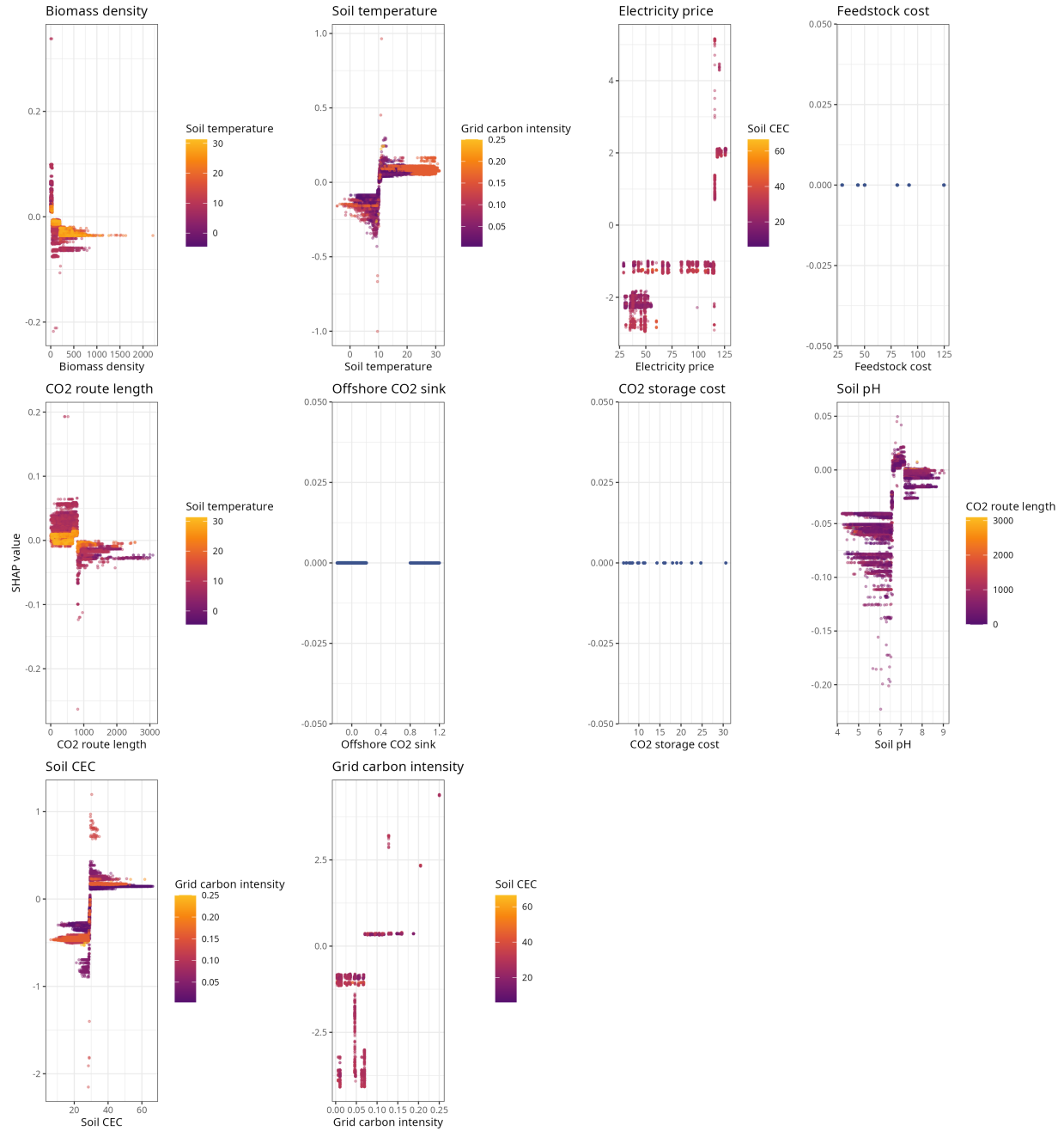
SHAP dependence, Global model: BES
