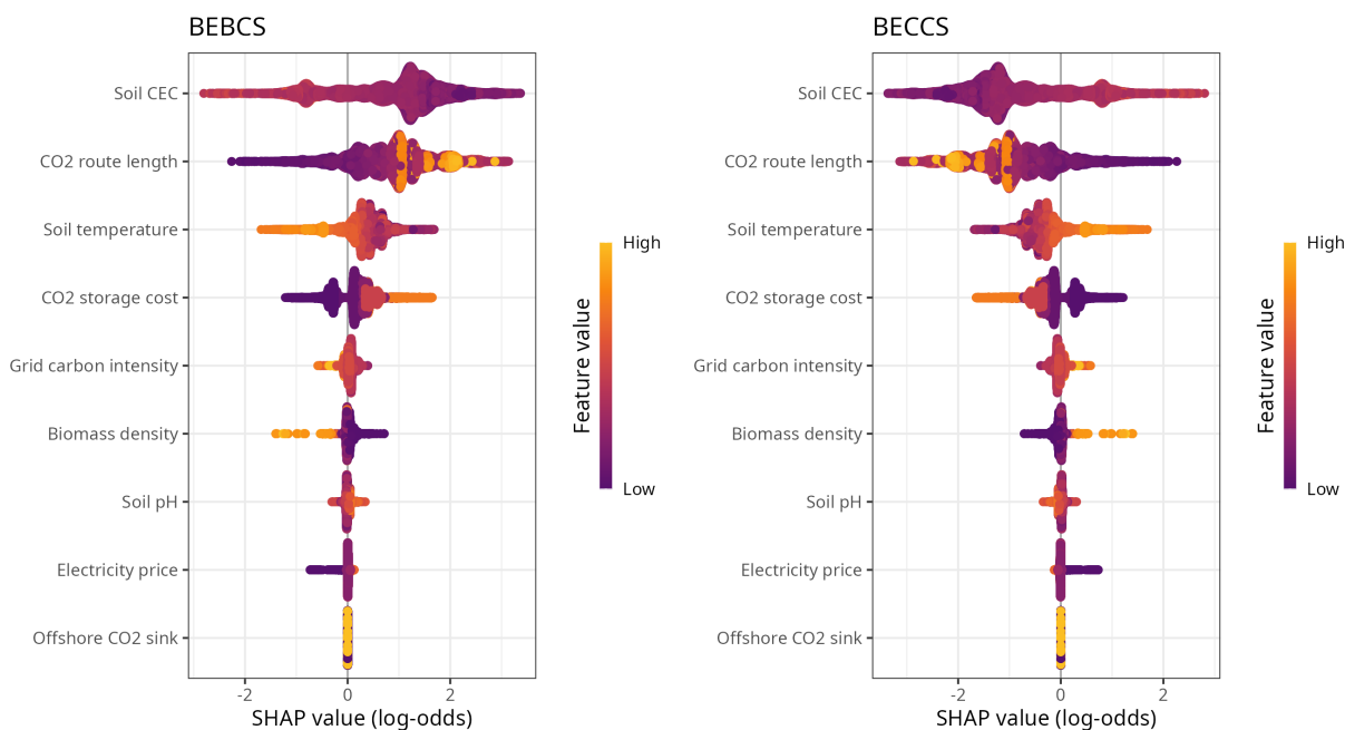
SHAP values for the optimal technology: US model
