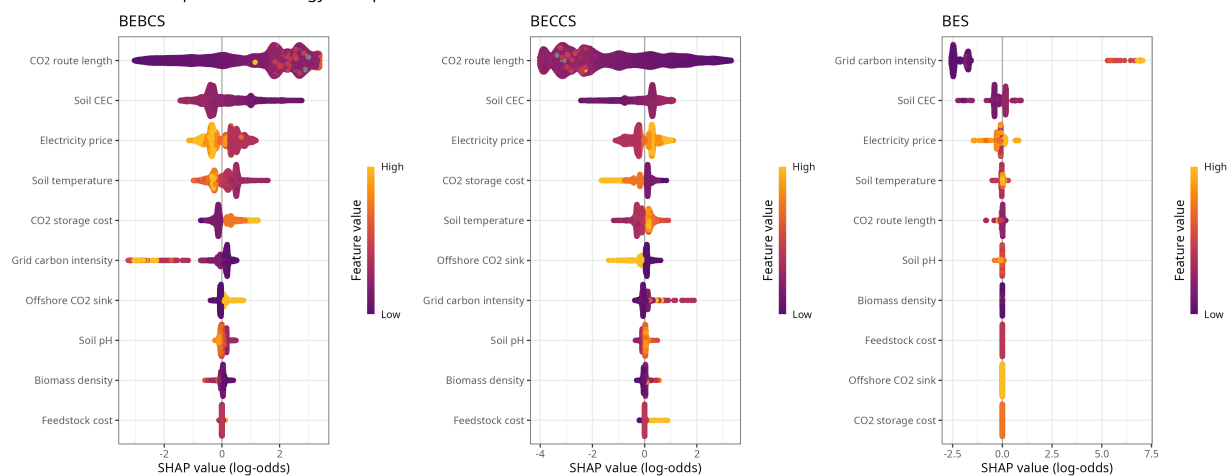
SHAP values for the optimal technology: Europe model
