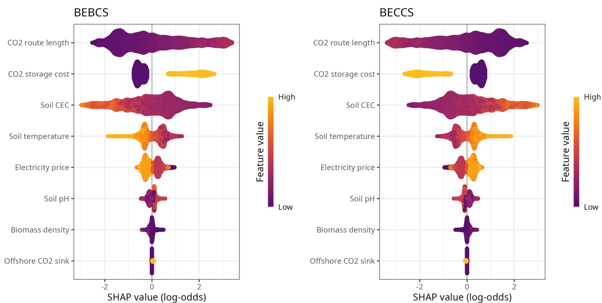
SHAP values for the optimal technology: China model
