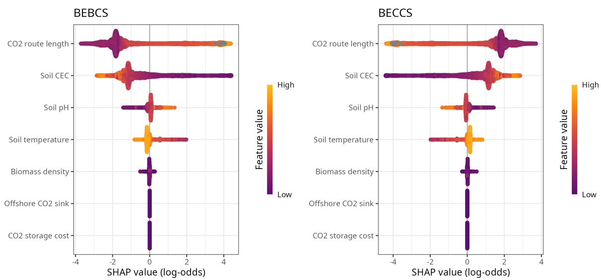
Figure S5: SHAP values by input, India model.
