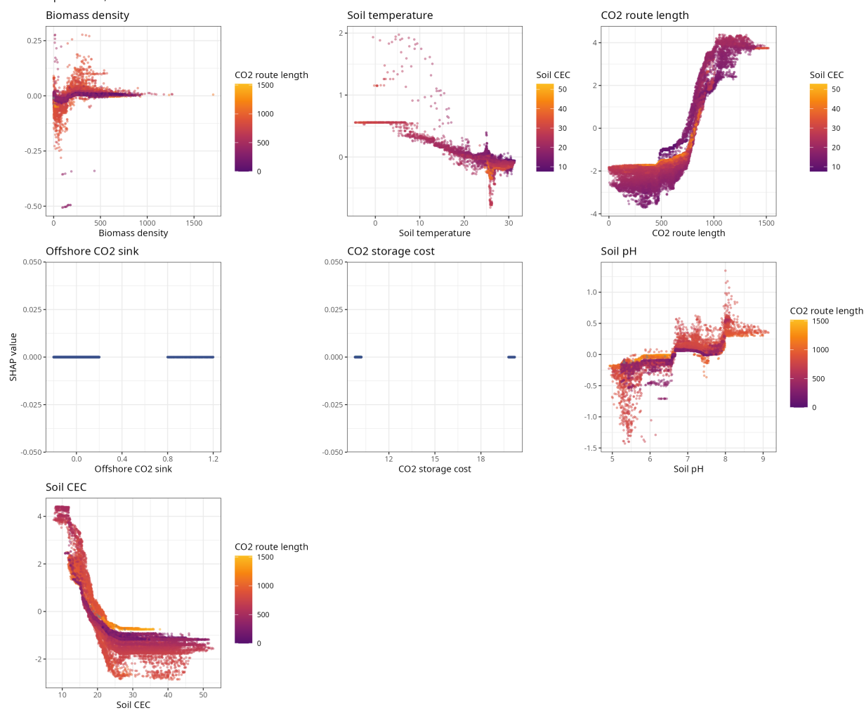
SHAP dependence, India model: BEBCS
