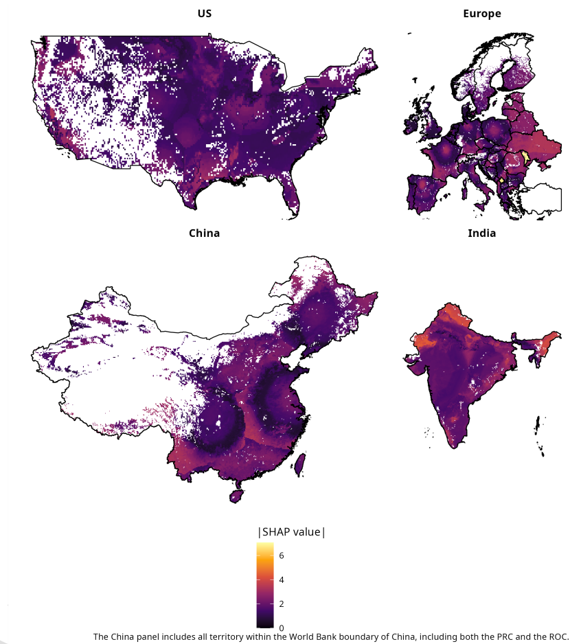
Figure 10: Magnitude (absolute SHAP value, log-odds) of the dominant spatial driver in each grid cell, from the regional surrogate classifiers. The China panel includes all territory within the World Bank boundary of China, including both the PRC and the ROC.
