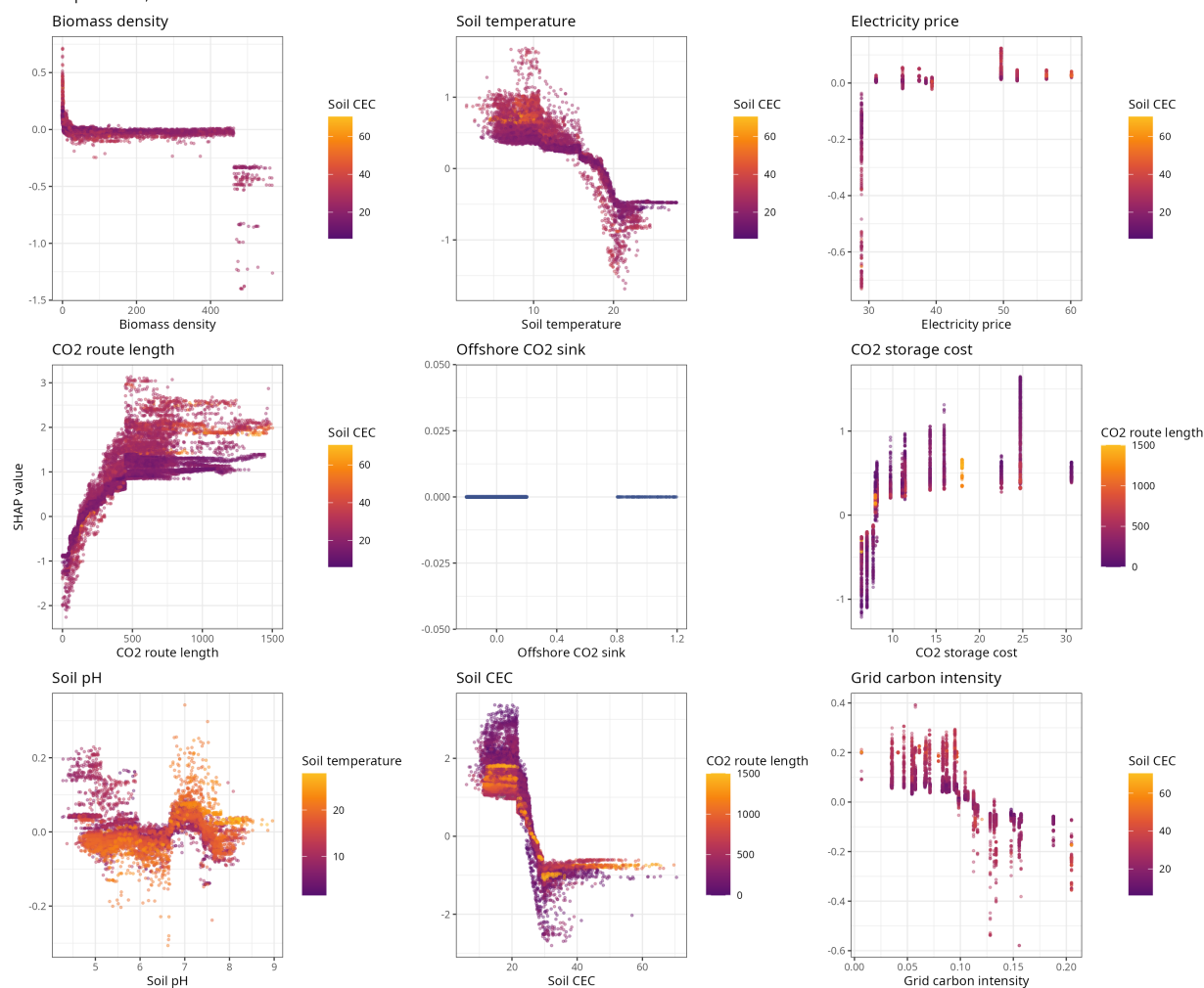
SHAP dependence, US model: BEBCS
