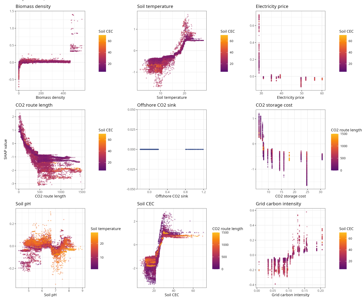
SHAP dependence, US model: BECCS
