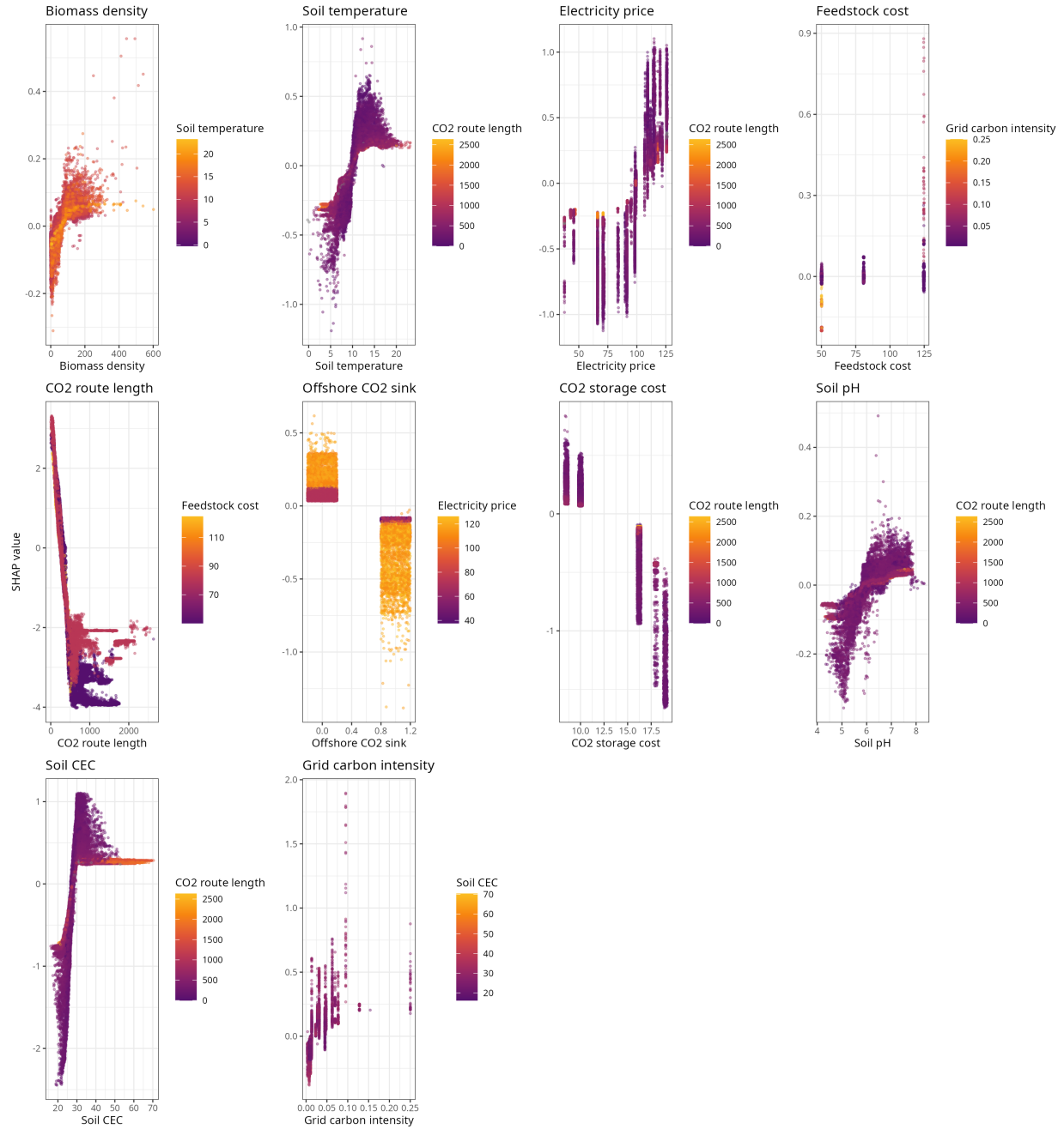
SHAP dependence, Europe model: BECCS
