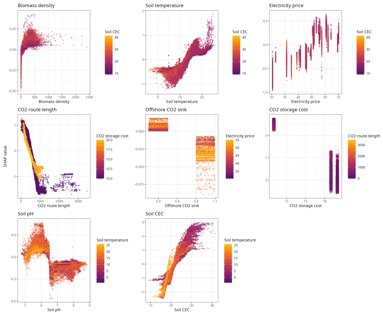
SHAP dependence, China model: BECCS
