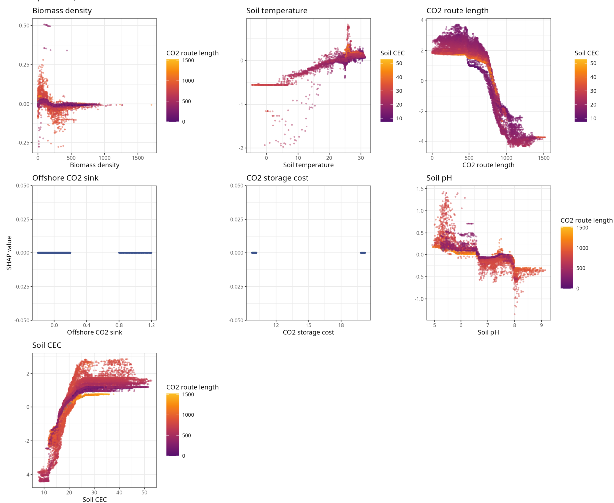
SHAP dependence, India model: BECCS
