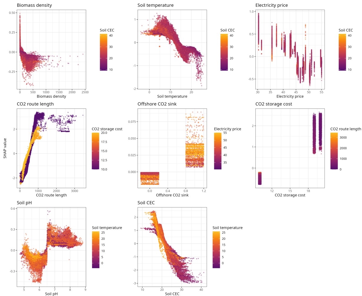
SHAP dependence, China model: BEBCS
