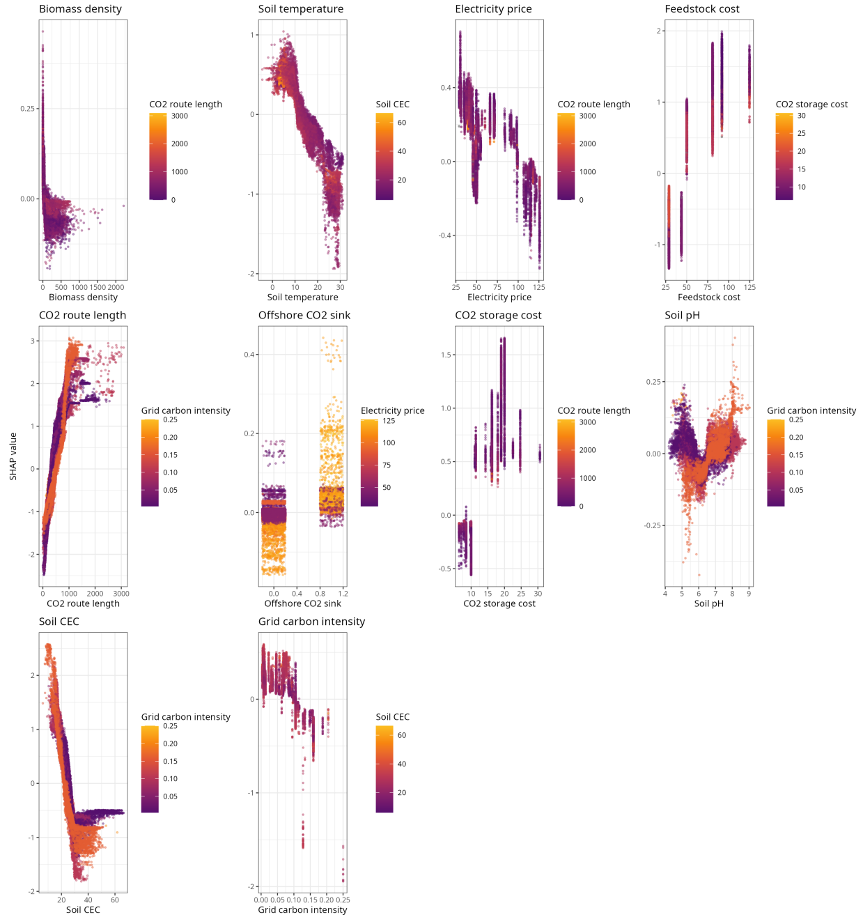
SHAP dependence, Global model: BEBCS
