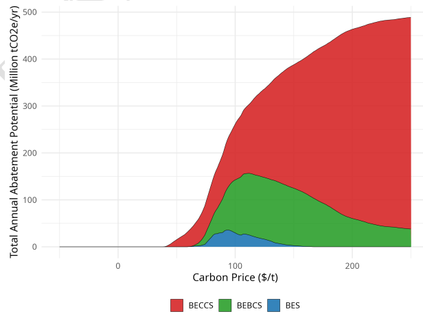
Figure 8: Marginal abatement cost curve for China. Land area is the total area of the grid cells assigned to each technology, not the cropland area within them.
