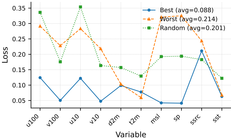
Per-variable validation loss
