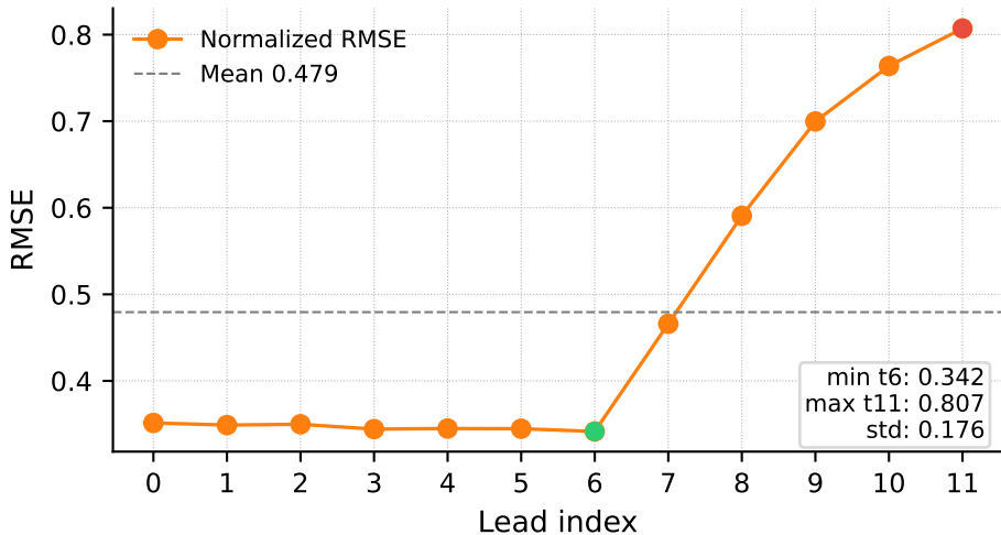
Normalized lead-wise pixel RMSE
