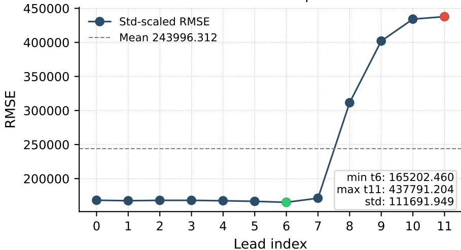
Std-scaled lead-wise pixel RMSE
