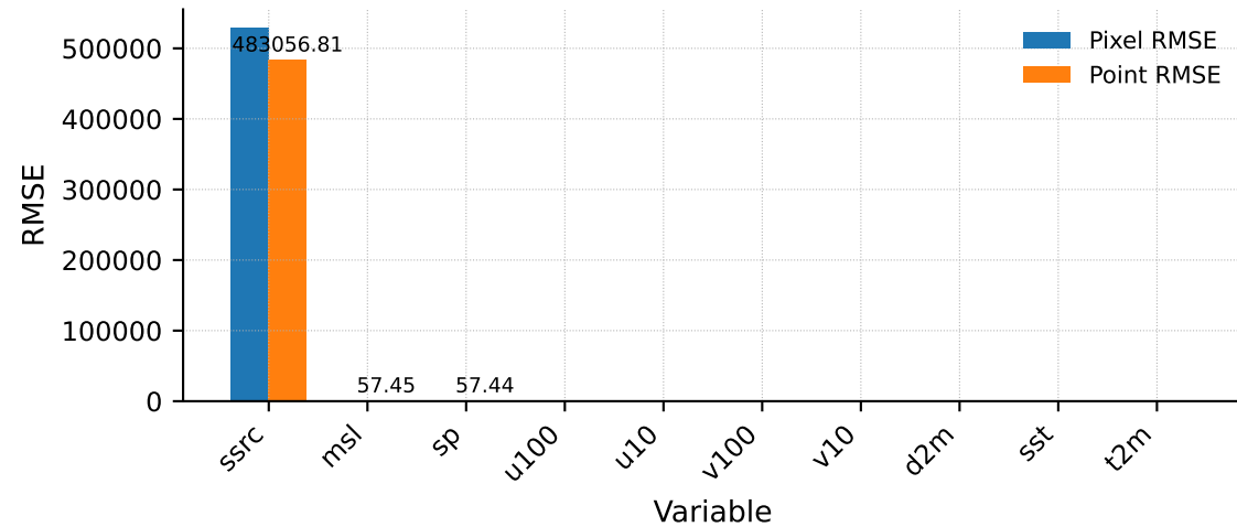
Per-variable RMSE (sorted by point error)
