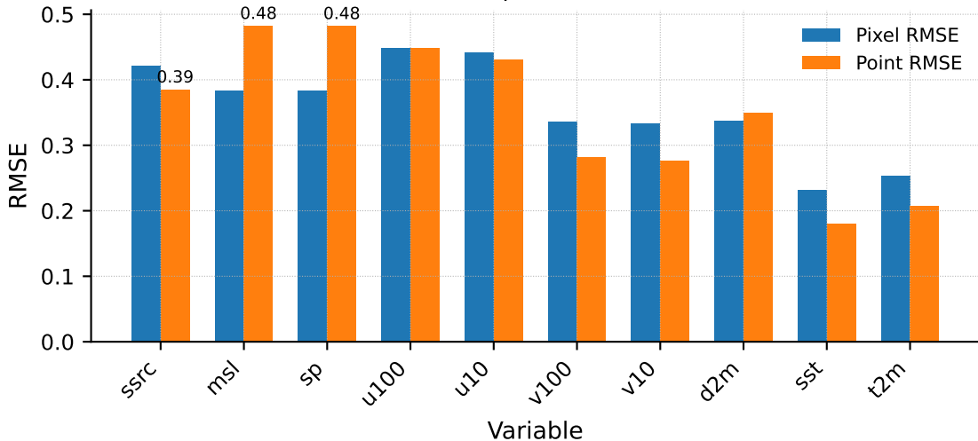
Normalized: per-variable RMSE
