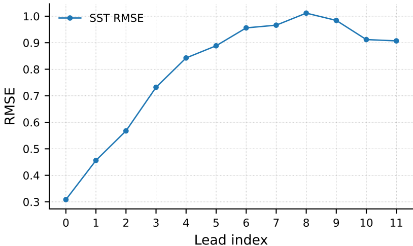
SST lead-time RMSE
