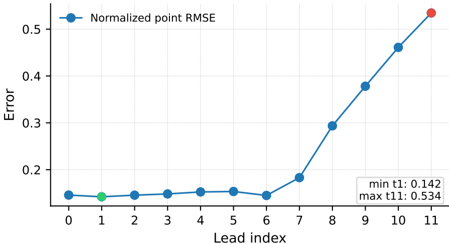
sst normalized point error by lead
