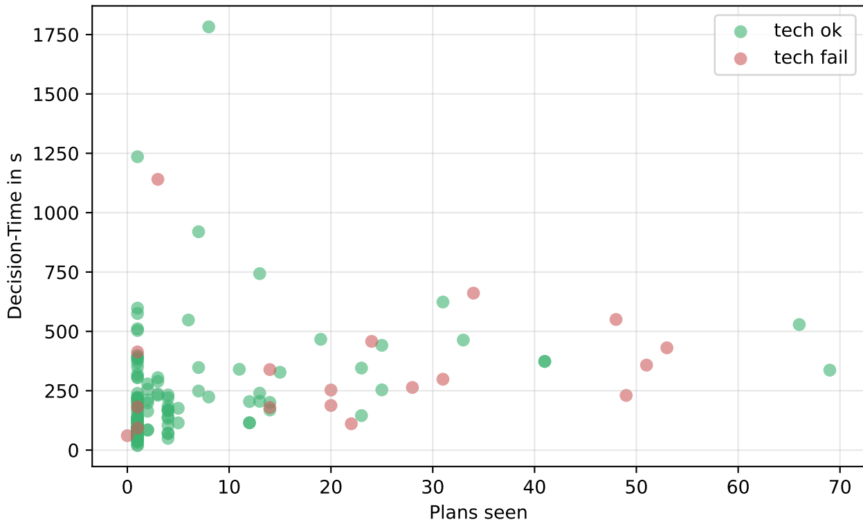
Plans vs Decision-Time, Spearman rho=0.49, p=0.000
