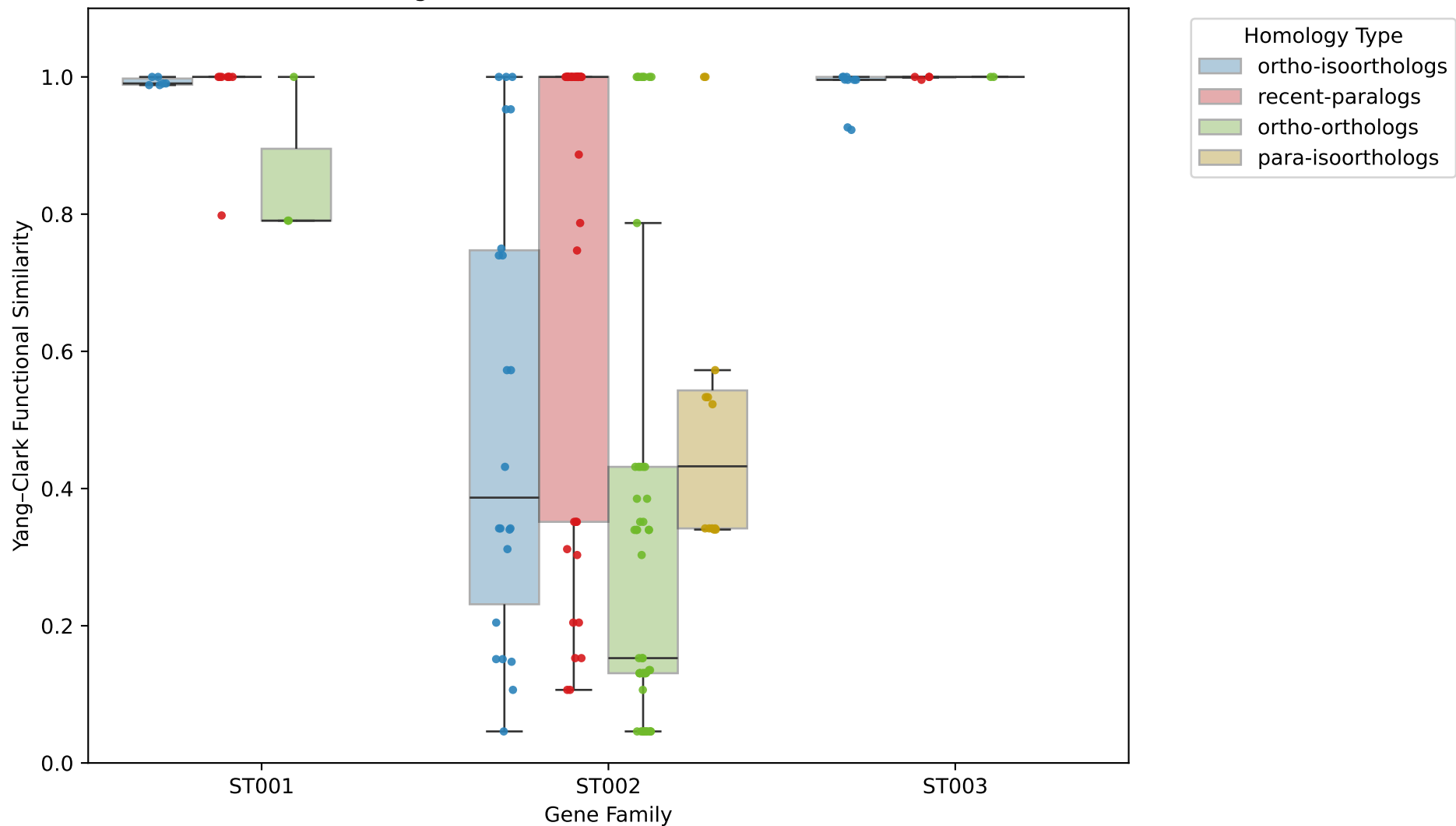
Distribution of Yang-Clark Functional Similarities: Molecular function
