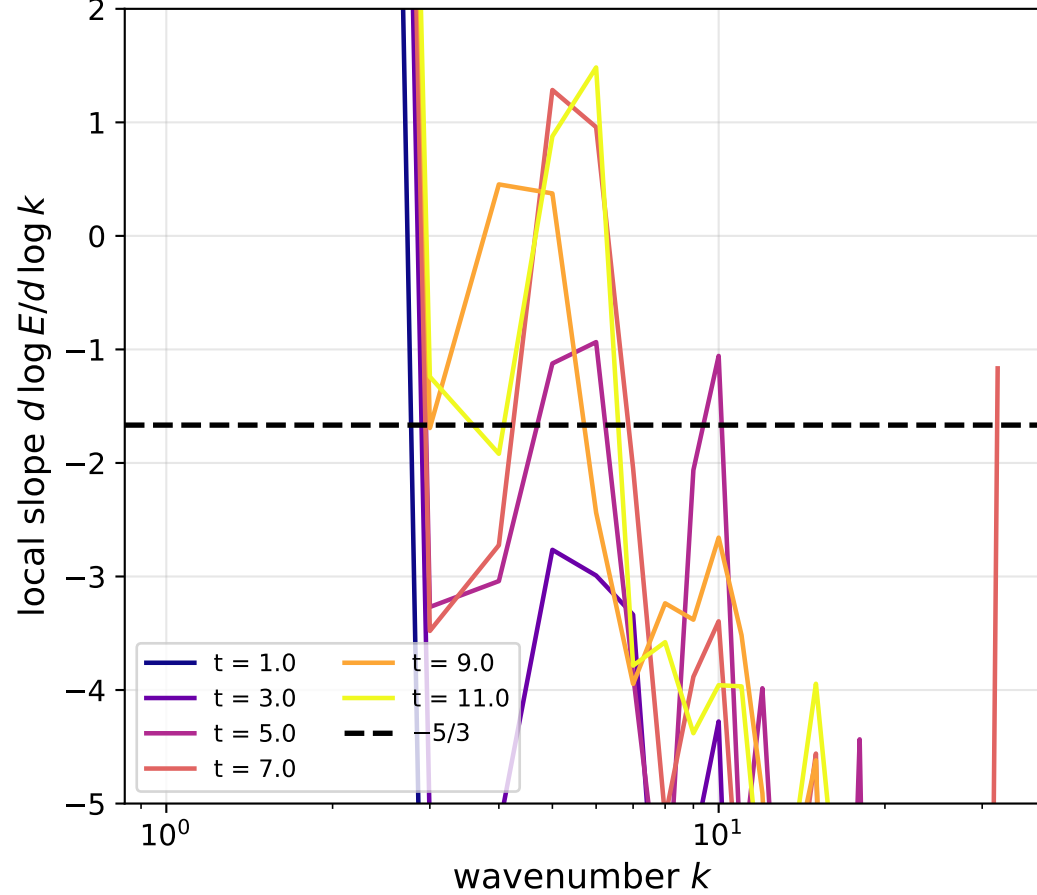
local spectral slope vs k (target -5/3 in inertial range)
