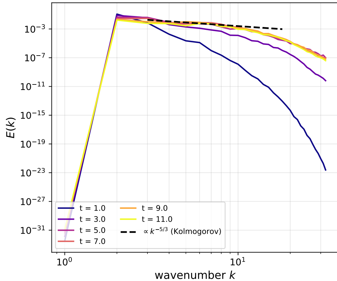
TGV Re=1600 on 64^3 , \nu_h = 2.5 \times 10^{-5} shell-averaged spectra
