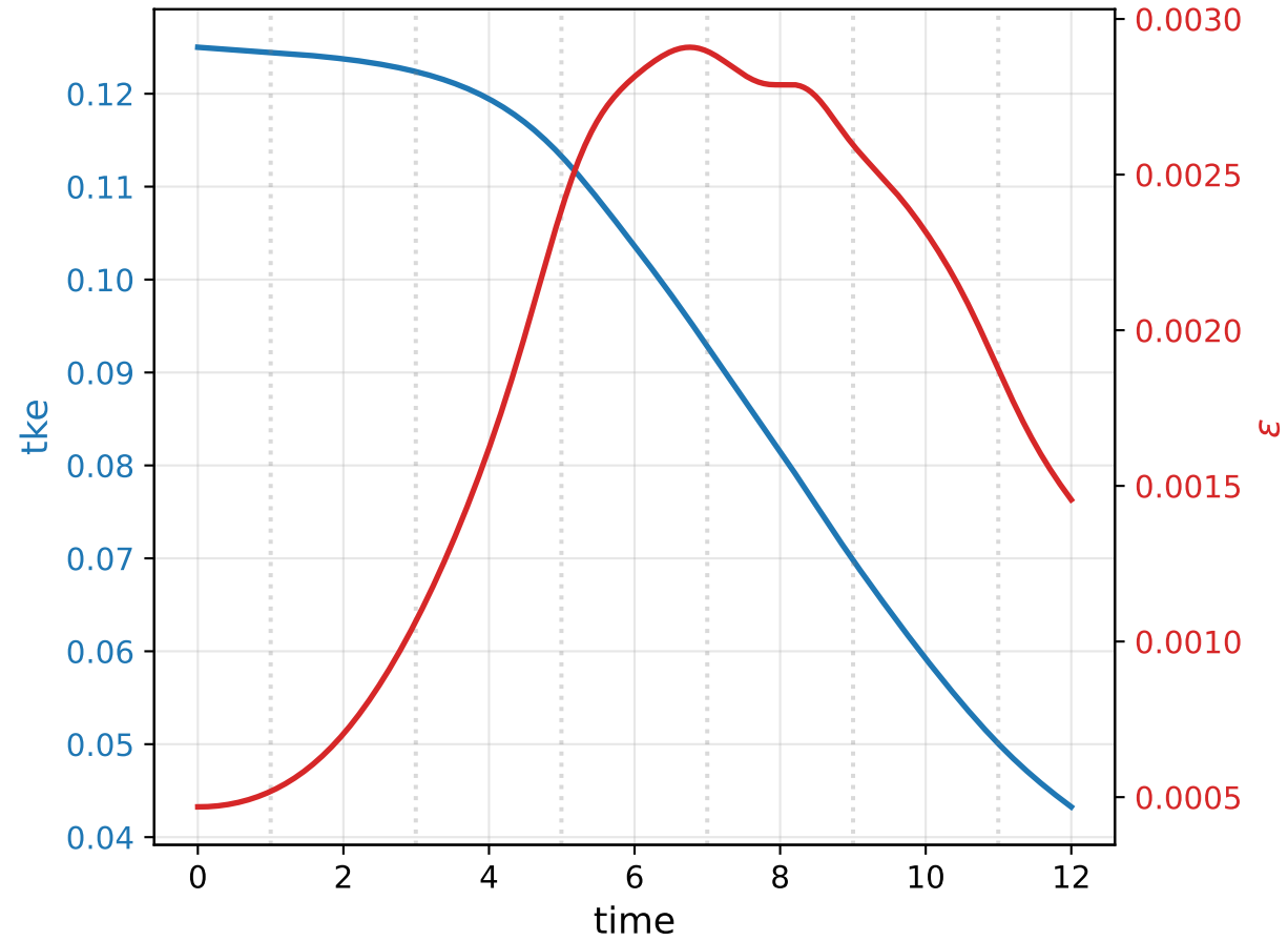
kinetic energy decay and dissipation
