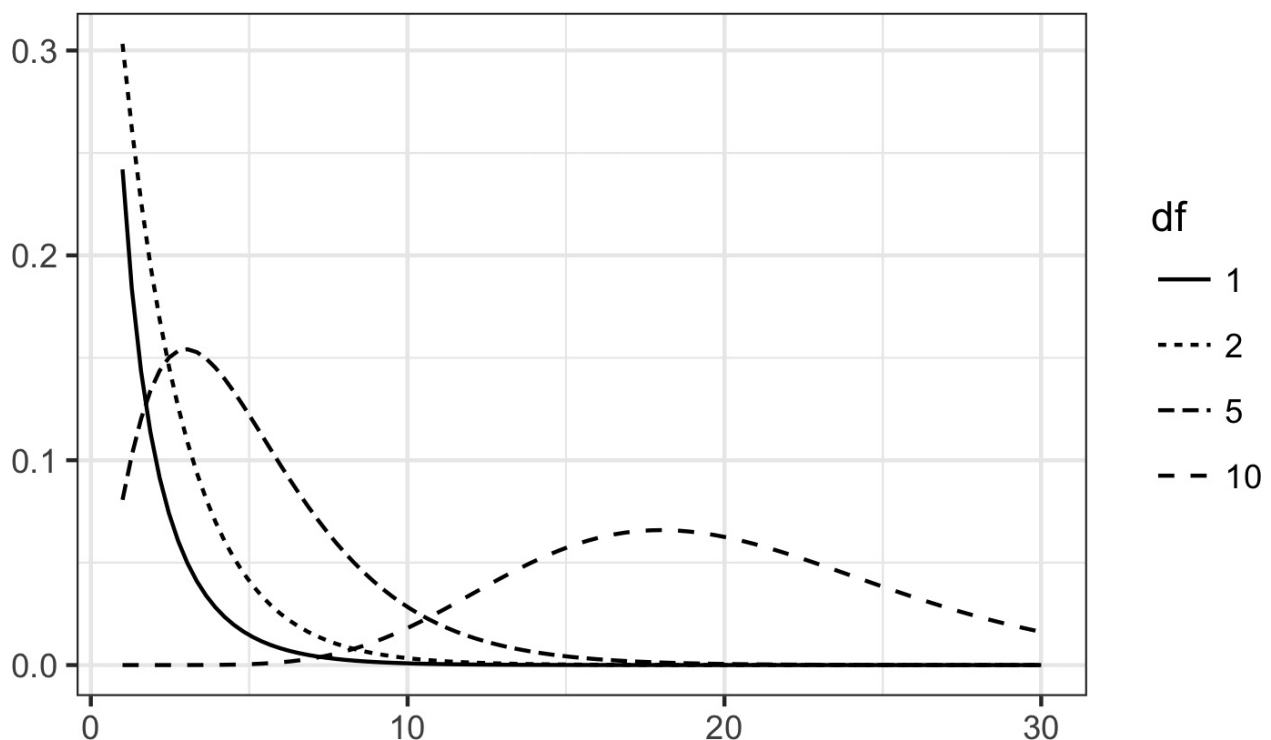
Figure 3-7. Chi-square distribution with various degrees of freedom (probability on y-axis, value of chi-square statistic on x-
