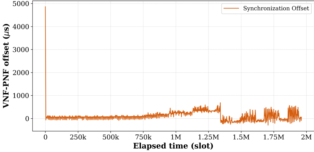
Figure 4.6: VNF-PNF synchronization offset over elapsed slots under the multi-switch/router deployment.
