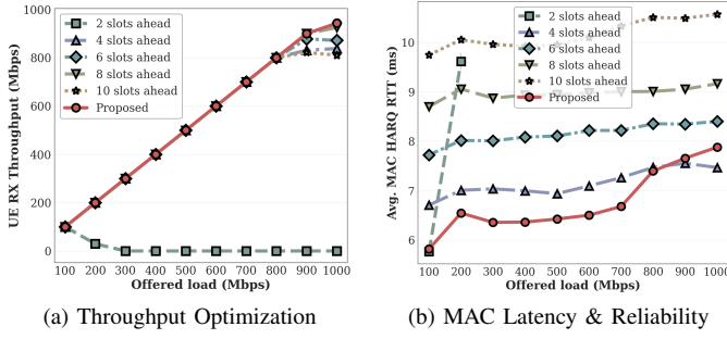
Fig. 5. Performance evaluation: MAC RTT efficiency and system throughput.
