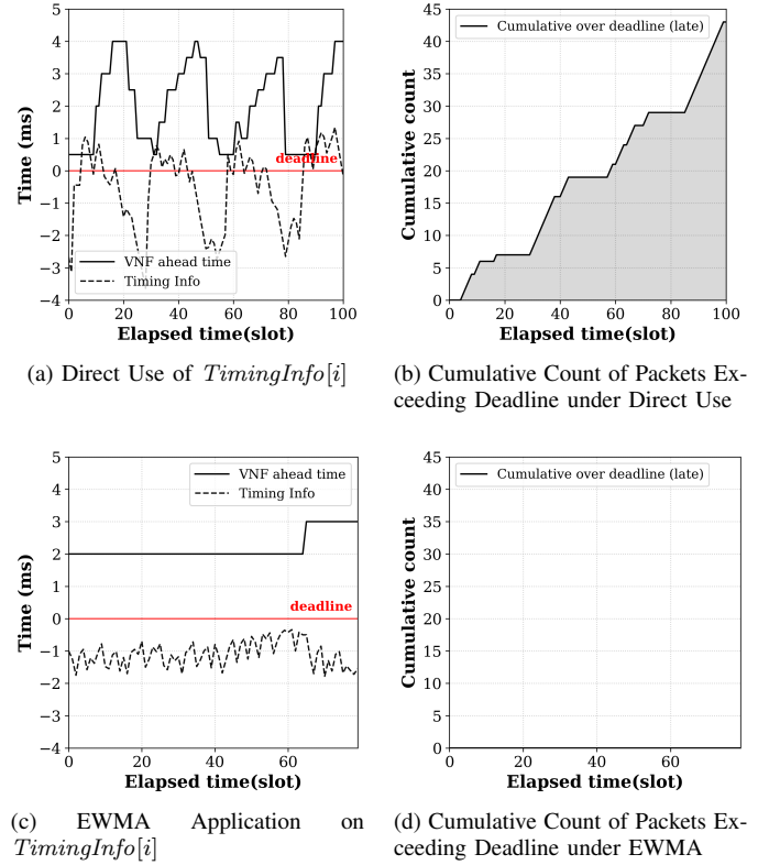
Fig. 4. Validation of EWMA processing on PNF Timing Info.
