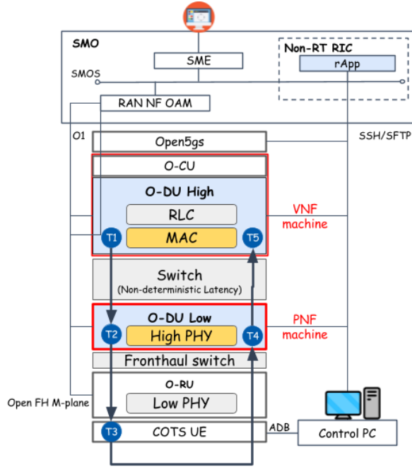
Fig. 2. Architecture of the rApp automated evaluation framework.
