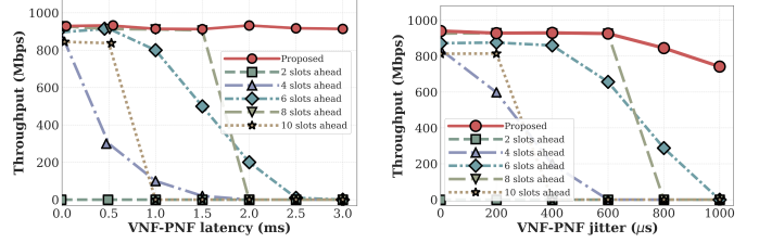
(a) Stability under Delay Congestion (b) Throughput under Unpredictable Jitter
