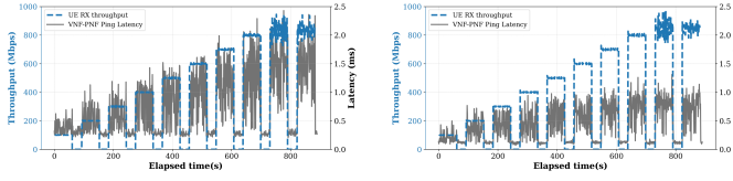
(a) Scenario II: Near-site deployment (b) Scenario III: Remote deployment
