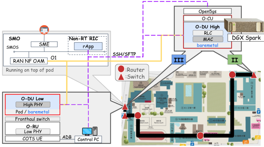
Figure 4.2: Experimental Scenario II: multi-switch/router campus deployment for evaluating the proposed adaptive timing control under realistic non-deterministic transport.
