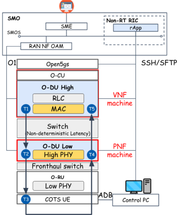
Fig. 2. Architecture of the rApp automated evaluation framework for Experimental Scenario I (Controlled Single-Switch setup with Linux TC delay injection).
