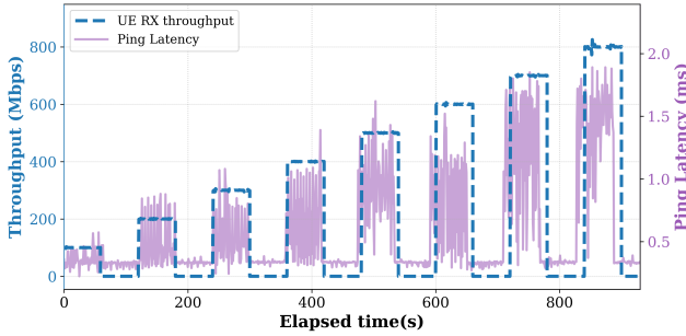
Fig. 7. UE RX throughput and ping latency under the multi-switch/router deployment.
