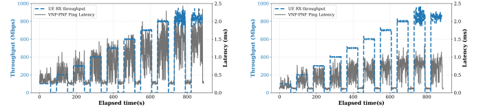
(a) Scenario II: Remote deployment (b) Scenario III: Near-site deployment
