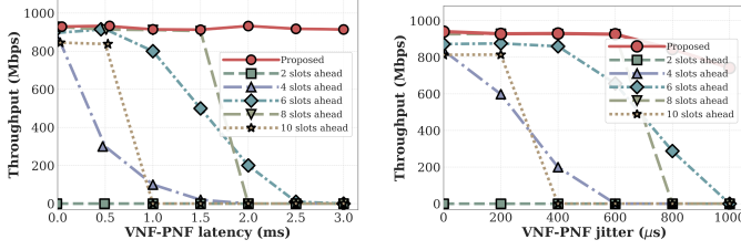
(a) Stability under Delay Congestion (b) Throughput under Unpredictable Jitter
