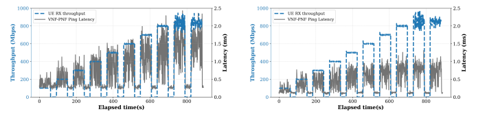
Fig. 8. UE RX throughput and ping latency under different real network deployment scenarios.
