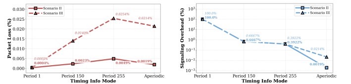
Fig. 9. Evaluation of packet loss rate under different deployment scenarios.
