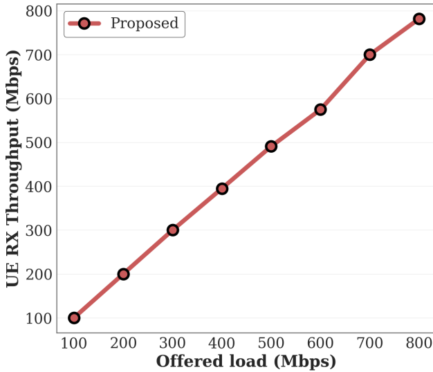
Fig. 7. UE RX throughput under the multi-switch/router deployment.
