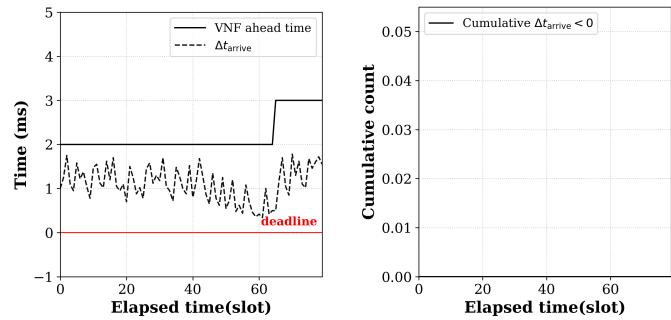
(c) EWMA Application on \Delta t_{arrive}
