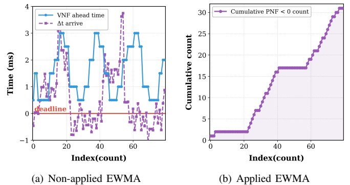
Fig. 3. Validation of EWMA processing on PNF Timing Info.
