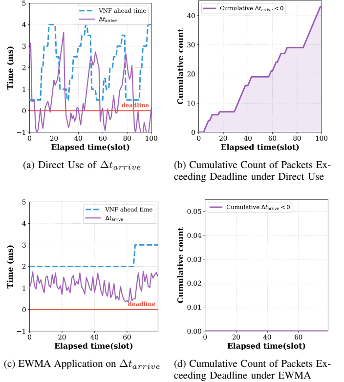
Fig. 3. Validation of EWMA processing on PNF Timing Info.
