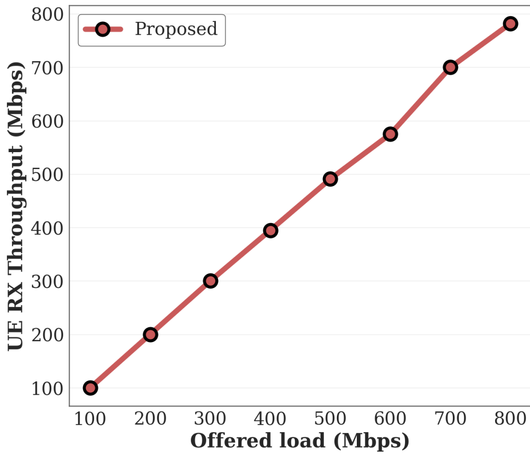
Figure 4.6: UE RX throughput under the multi-switch/router deployment.
