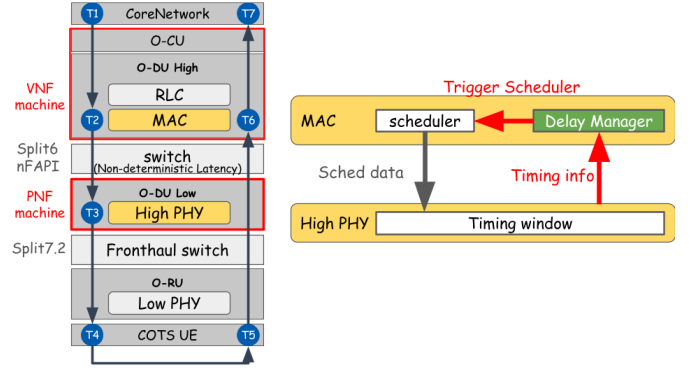
Fig. 1. System architecture and delay management mechanism.
