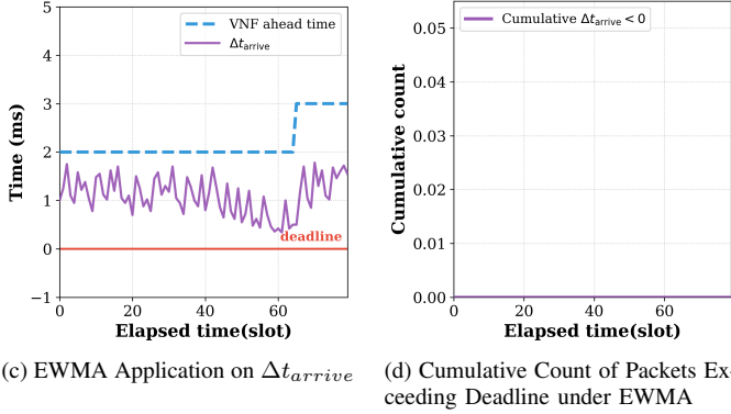
Fig. 4. Validation of EWMA processing on PNF Timing Info.
