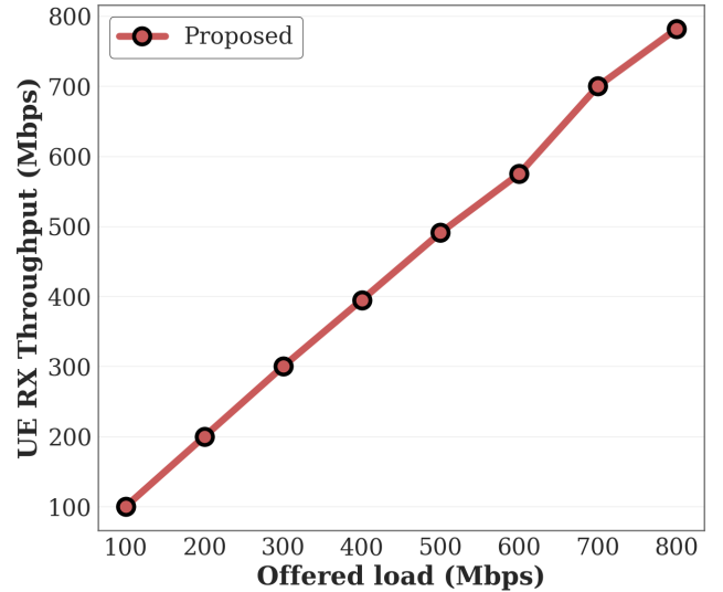
Fig. 7. UE RX throughput under the multi-switch/router deployment.
