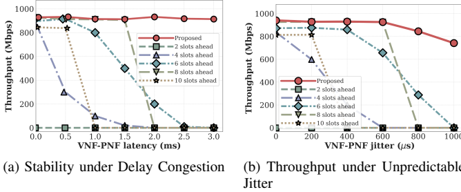
Fig. 6. System stability and throughput performance under varying network conditions.
