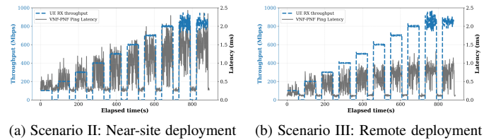
Fig. 8. UE RX throughput and ping latency under different real network deployment scenarios.
