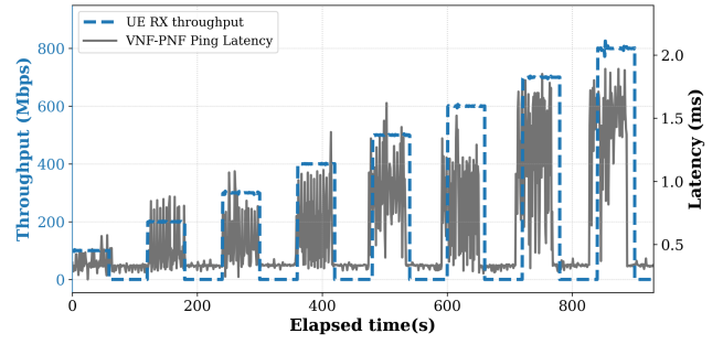
Fig. 8. UE RX throughput and ping latency under the multi-switch/router deployment.
