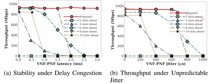
Fig. 6. System stability and throughput performance under varying network conditions.
