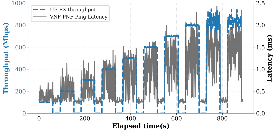
(a) UE RX throughput and ping latency over a continuous timeline
