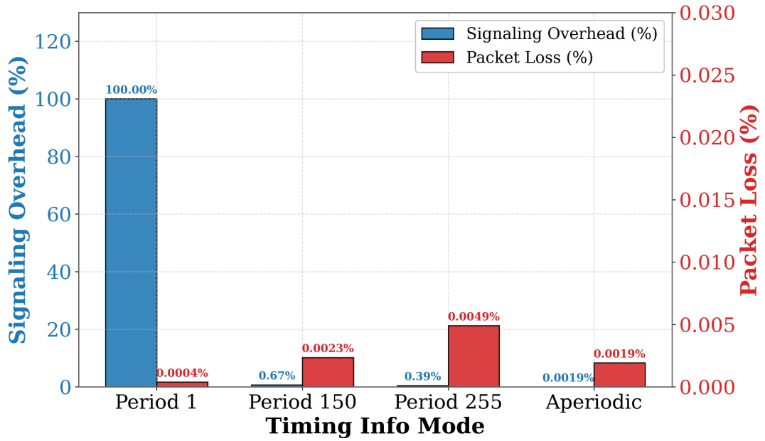
(b) Packet loss rate under different timing info reporting periods
