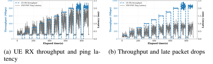
Fig. 8. System performance and latency under real network congestion.
