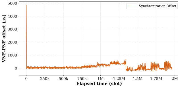
Fig. 7. VNF-PNF synchronization offset over elapsed slots under the multi-switch/router deployment.
