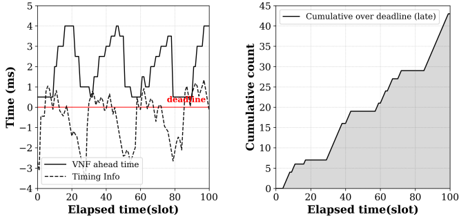
(a) Direct Use of TimingInfo[i]
