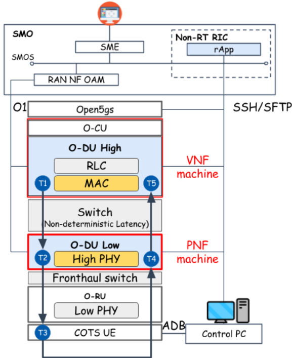
Fig. 2. Architecture of the rApp automated evaluation framework.
