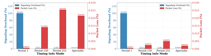
Fig. 9. Evaluation of packet loss rate under different timing info modes and periods.
