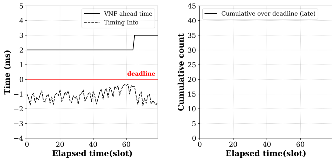
(c) EWMA Application on TimingInfo[i]
