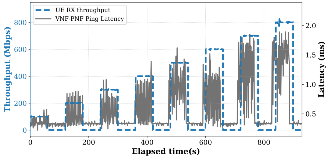
Figure 4.7: UE RX throughput and ping latency over a continuous timeline under the multi-switch/router deployment.
