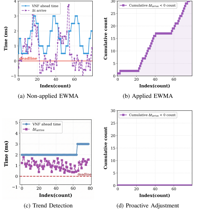
Fig. 4. Validation of EWMA processing on PNF Timing Info and proactive adjustment.
