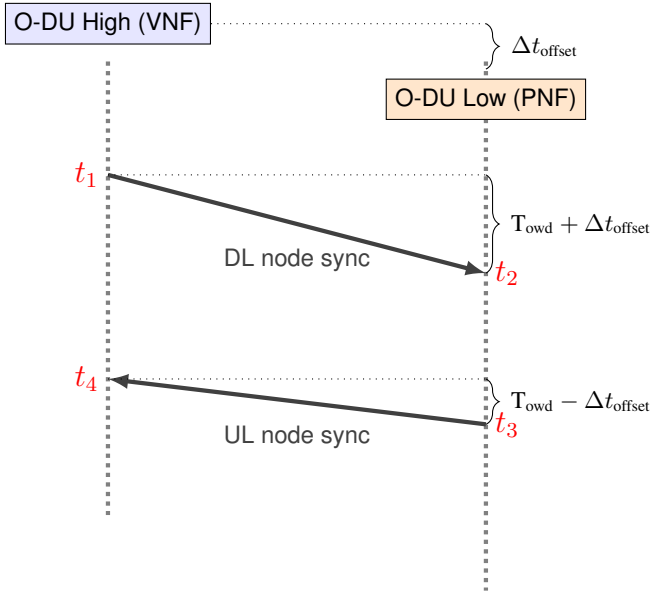
Fig. 3. Delay Management Procedure (Node Sync)
