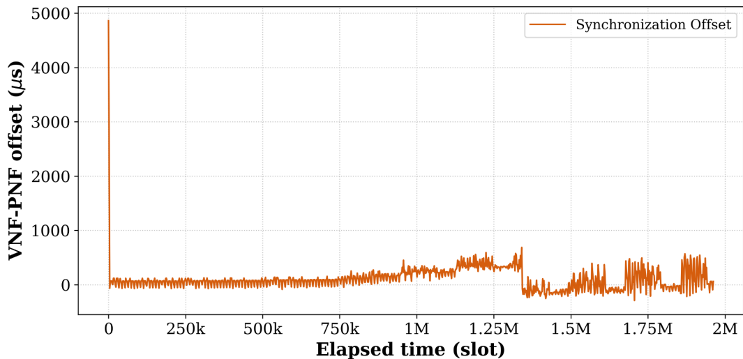
Figure 4.6: VNF-PNF synchronization offset over elapsed slots under the multi-switch/router deployment.
