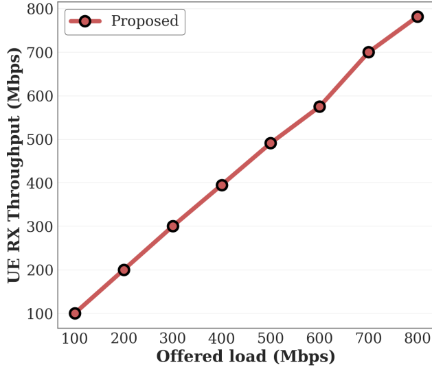
Fig. 7. UE RX throughput under the multi-switch/router deployment.
