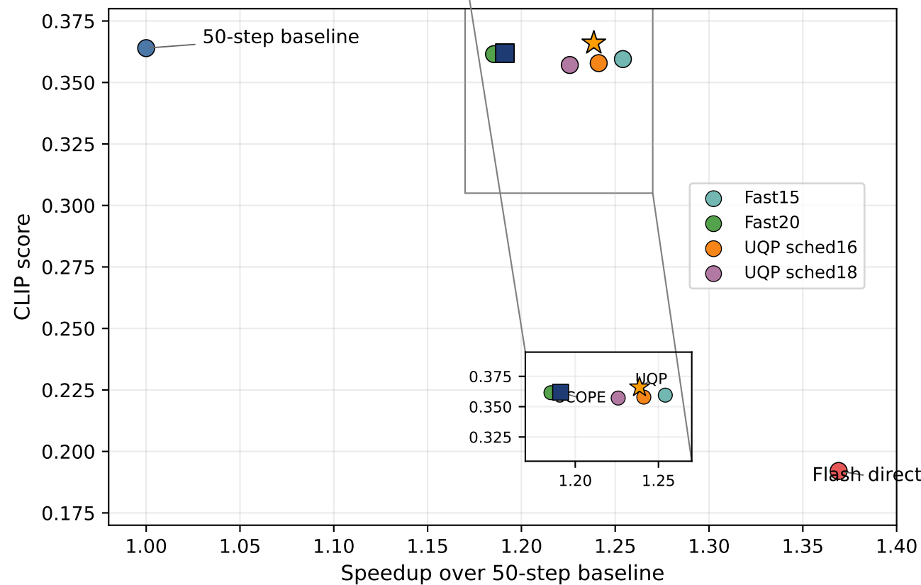
Generation trade-off
