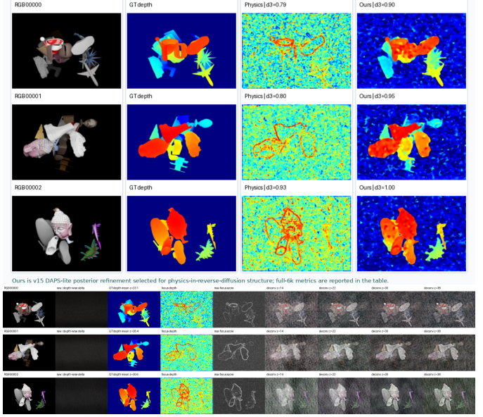
Fig. 2. Result panels. Top: clean v15 DAPS-lite depth examples with RGB, GT depth, physics focus baseline, and Ours ; teacher and error-map panels are omitted. Bottom: mid/late PSF-Wiener deconvolution planes z = \{14, 22, 30, 38\} , which avoid unstable early-plane inverses while showing depth-dependent focus.
