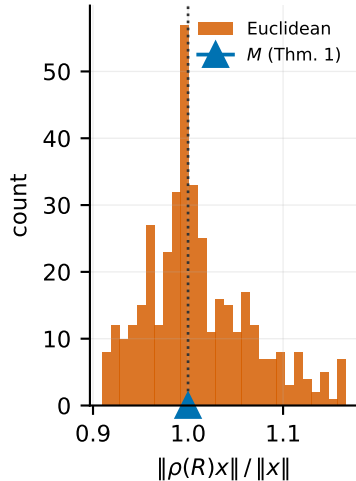
(c) the action is not orthogonal
