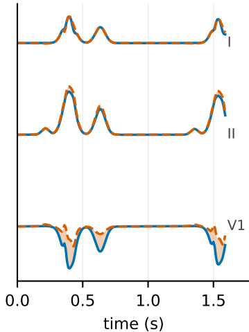
(b) x (solid) vs \rho(R)x (dashed)
