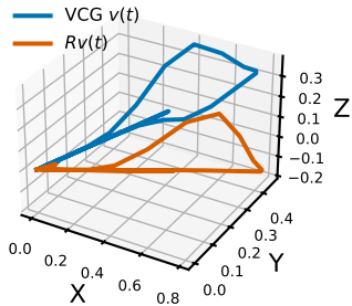
(a) heart vector
