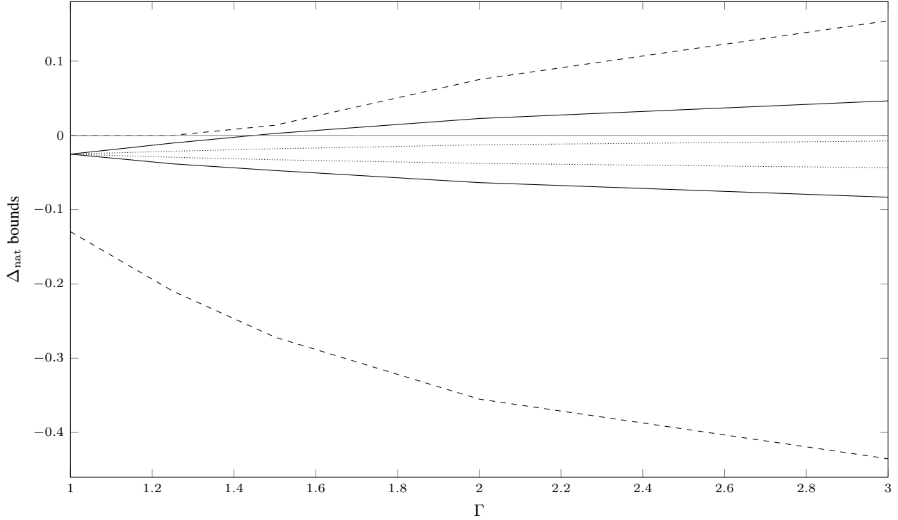
Figure 1. Lower and upper bounds of \Delta_{\text{nat}} versus \Gamma for settings A (dotted), C (solid) and B (dashed); MCAR truth (P2-FR2-B).
