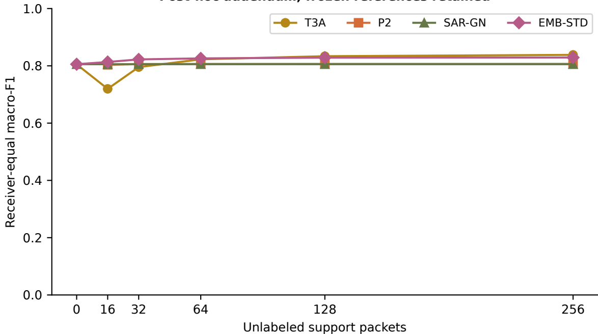
Support budgets: common 256-reserve query set Post-hoc addendum; frozen references retained
