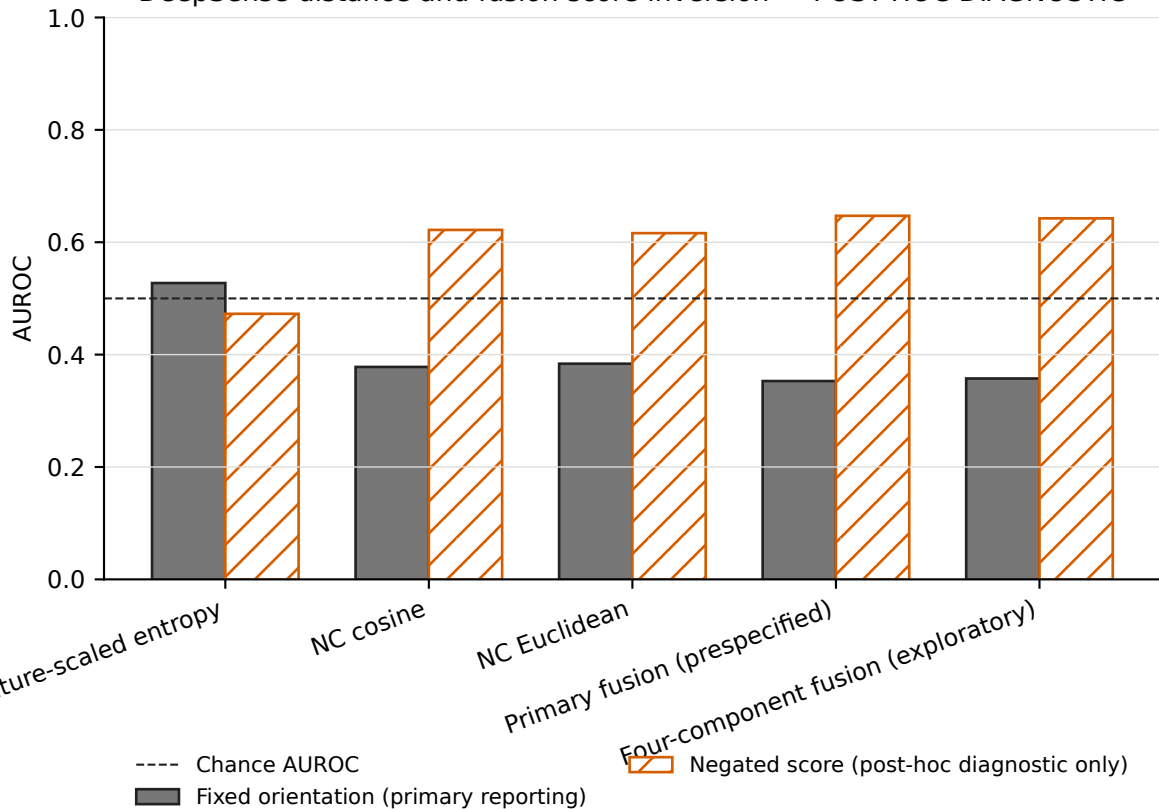
DeepSense distance and fusion score inversion — POST-HOC DIAGNOSTIC
