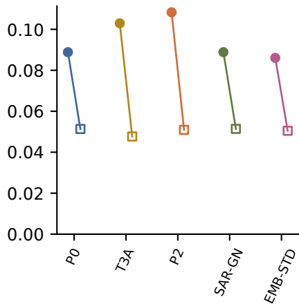
ECE (lower is better)
