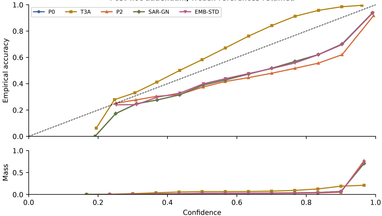
Raw reliability: pooled descriptive bin counts (not packet inference) Post-hoc addendum; frozen references retained
