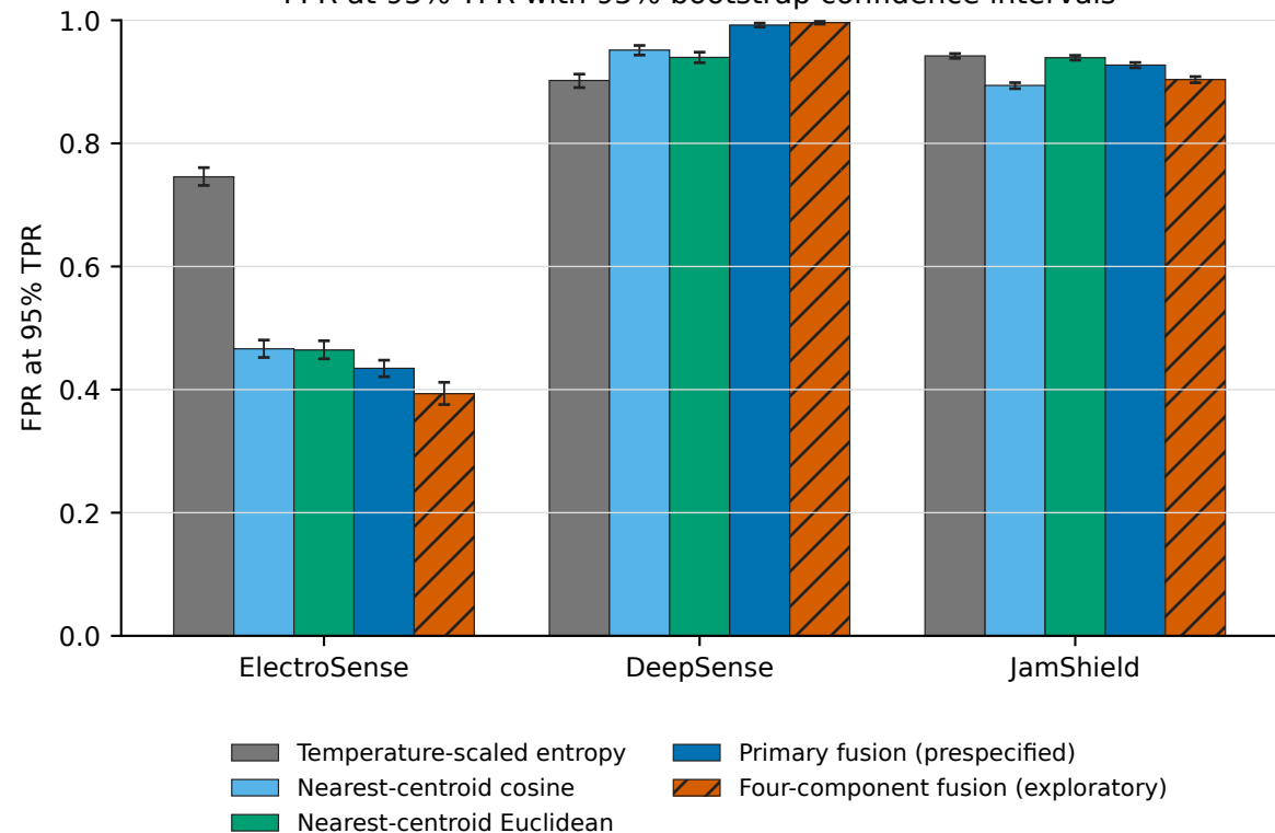
FPR at 95% TPR with 95% bootstrap confidence intervals
