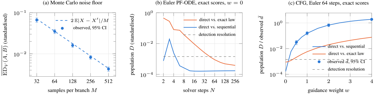
Figure 1. Separating numerical components on the Gaussian probe. (a) The Monte Carlo floor of the V-statistic energy distance between two independent sets follows 2\mathbb{E}|X - X'|/M (P5-E5, N = 200 ). (b) With exact scores and no guidance, the closed-form gap between the direct and sequential PF-ODE laws falls below the one-sided 5% detection resolution of the v1 design ( N = 100 , M = 256 ) from about 6 steps on, and plateaus at the prior-mismatch value, although the sampler remains biased relative to the exact law. (c) Guidance alone creates direct-vs-sequential gaps far above the resolution; the observed means (P5-E7) match the closed form. Closed-form curves are computed from the affine output law (Proposition 4.4); no Monte Carlo is involved in them.
